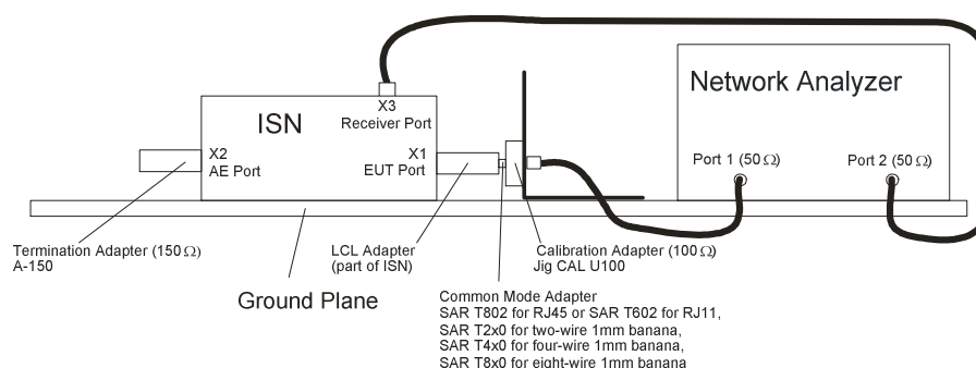
Fig. 8 Test set-up for Voltage Division Factor in accordance with CISPR 16-1-2
