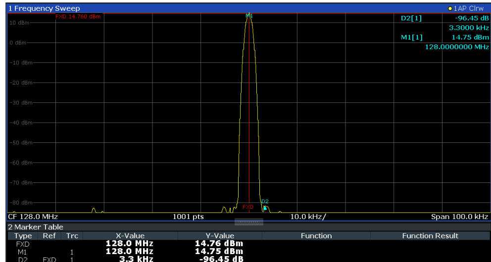
Figure 5-16: Fundamental wave and the frequency and level reference point
