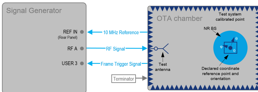
Figure 8-2: One path test setup (example of R&S SMM100A simulating the test case 7.4 "OTA dynamic range")
