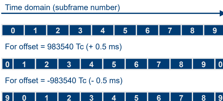
Figure 5-2: Example: Timing advance offset in a frame
