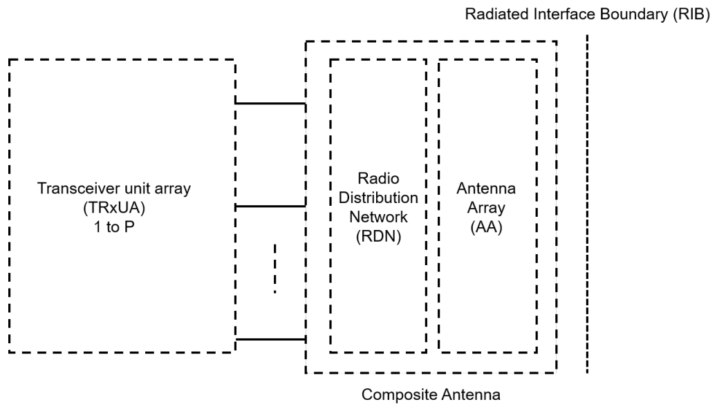
Figure 8-3: Radiated reference points for BS type 1-O and BS type 2-O as defined in TS 38.141-2
