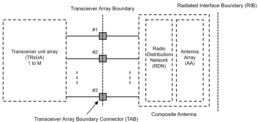
Figure 8-4: Radiated and conducted reference points for BS type 1-H as defined in TS 38.141-2
