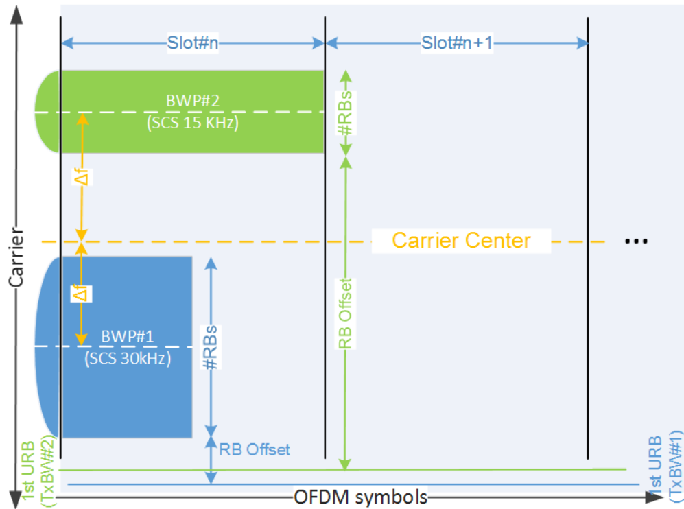
Figure 5-4: Bandwidth parts
