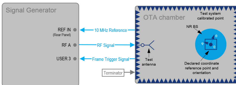
Figure 8-2: One path test setup (example of R&S SMM100A simulating the test case 7.4 "OTA dynamic range")
