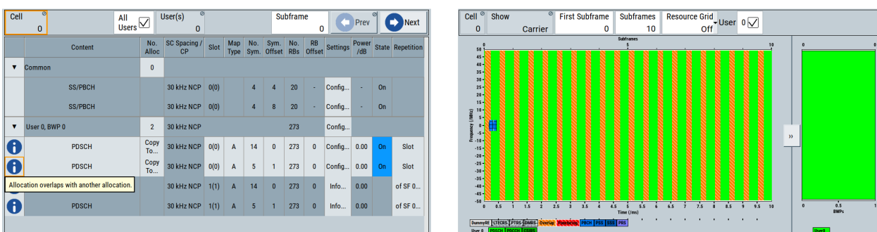
Figure 2-7: Overlapping allocations
