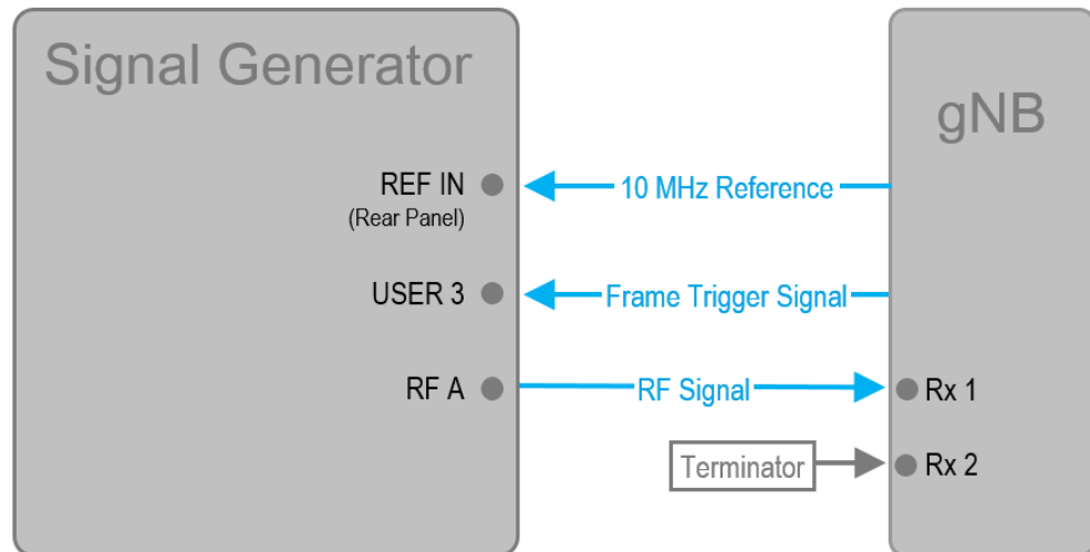
Figure 8-1: One path test setup (example of R&S SMM100A simulating the test case 7.3 "Dynamic range")
