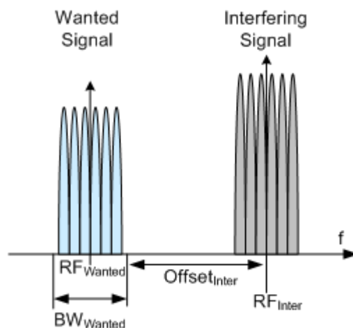
Figure 8-7: Example: adjacent channel selectivity (ACS)
