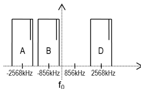
Figure 2-7: Three channel T-DMB signal
