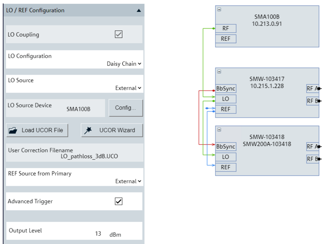
Figure 3-16: LO / REF configuration and its graphical representation
