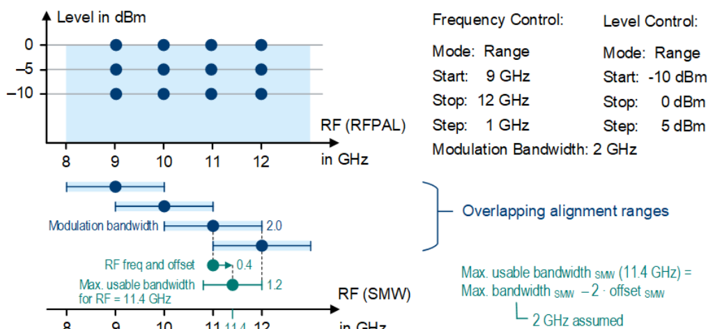
Figure 3-9: Calibration set and relations to the RF signal at the R&S SMW
