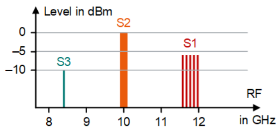
Figure 3-11: Signals to be aligned
