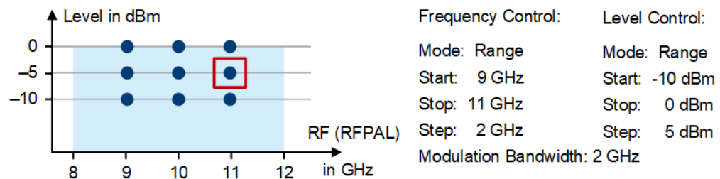
Figure 3-12: Calibration set (highlighting corresponds to the following figure)
