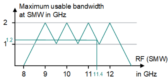
Figure 3-10: Maximum usable bandwidth for the RF signal at the R&S SMW
