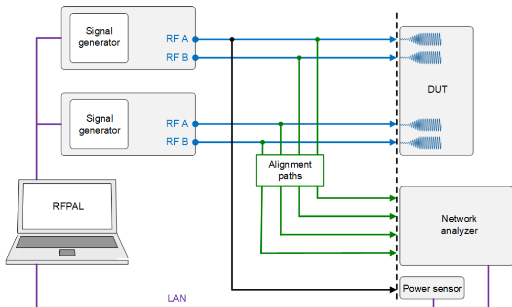
Figure 3-1: RF paths to be aligned
