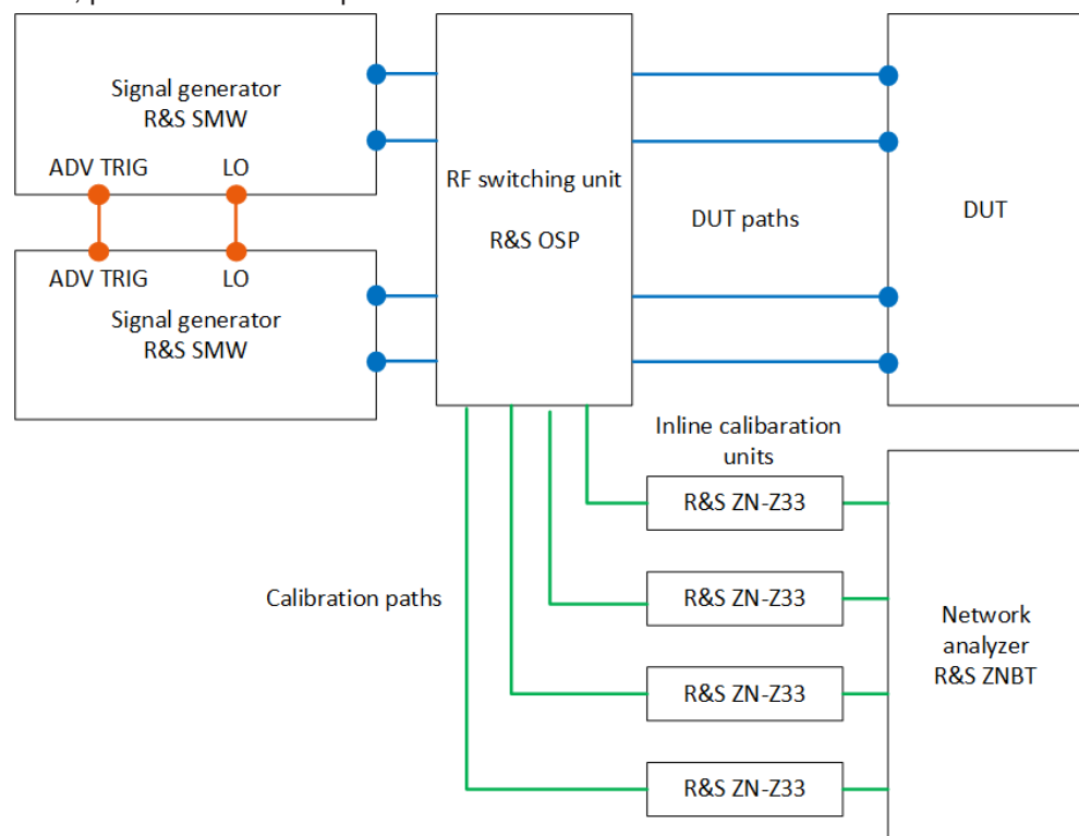
Figure 3-8: Example: test setup with inline calibration units
