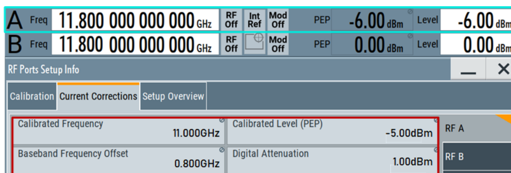
Figure 3-13: Settings and calibration parameters at the R&S SMW for Signal S1
