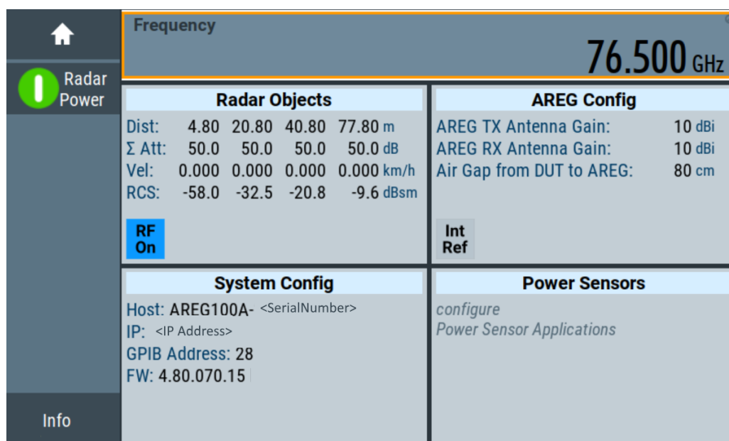
Figure 3-3: Touchscreen
