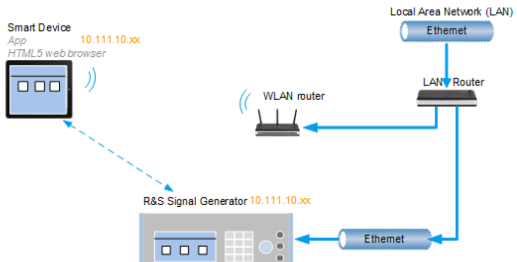
Figure 9-9: Example of a network configuration for remote operation with a smart device
