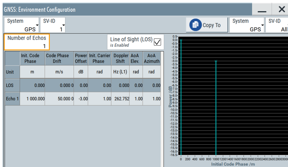
Figure 8-5: Static multipath configuration for GPS space vehicles
