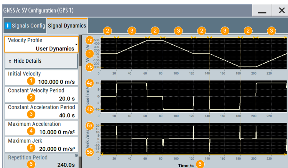
Figure 11-1: Understanding high-order user-defined signal dynamics
