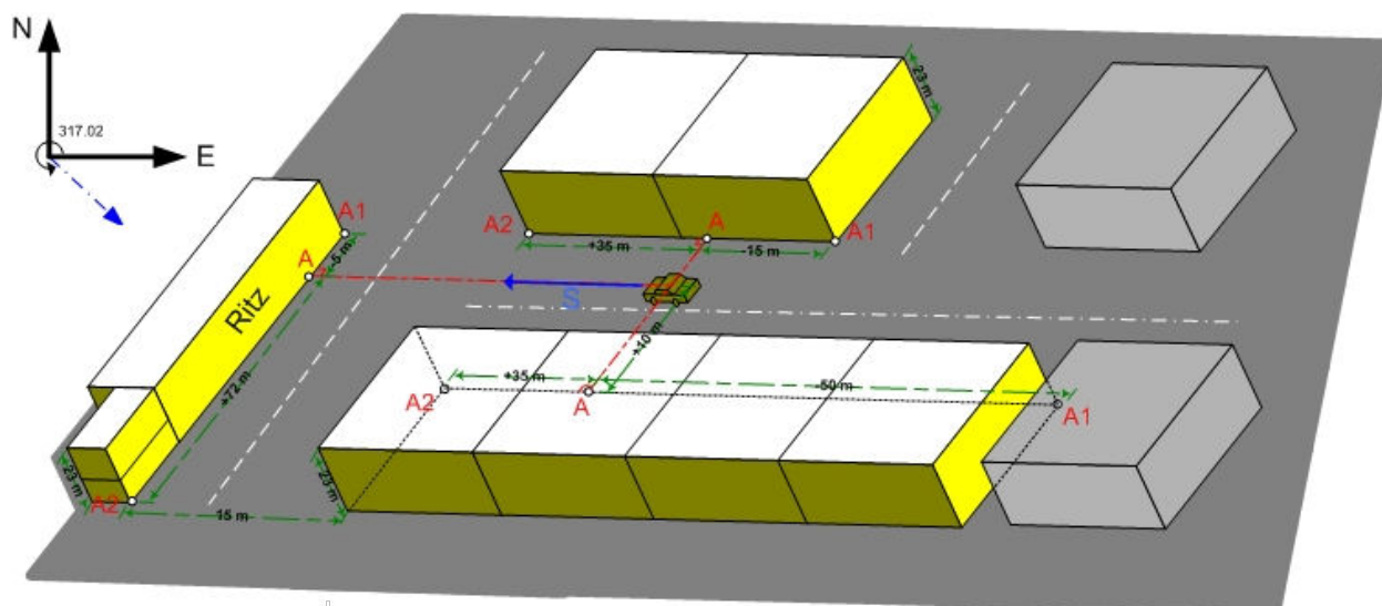
Figure 8-4: Example: Vertical obstacles for simulation of obscuration and multipath from surrounding buildings
