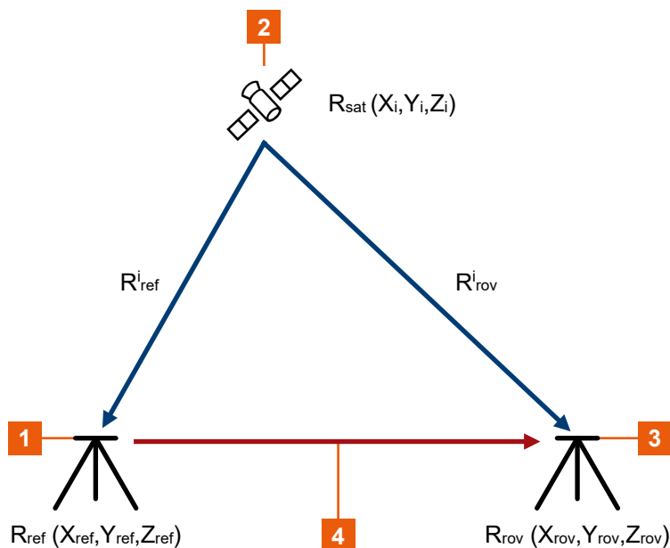
Figure 9-1: RTK principle
