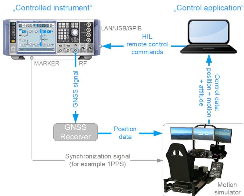
Figure 19-1: Example of HIL test setup
