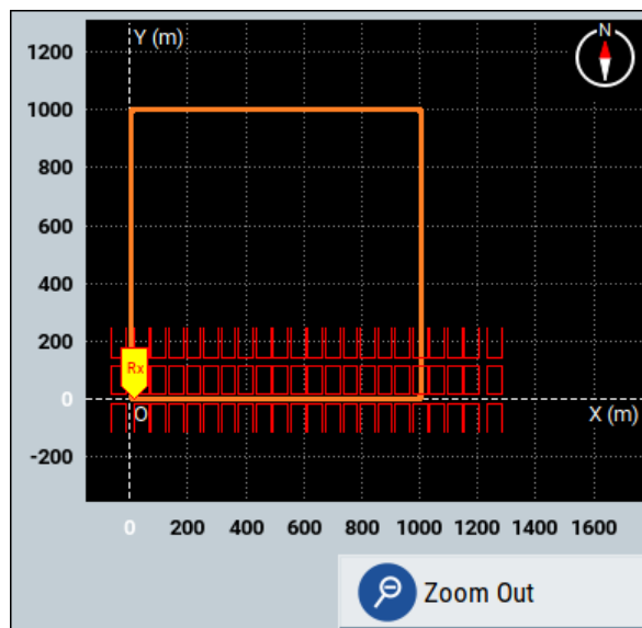
Figure 8-7: Obstacles file graphic: Obstacle position, receiver position (Rx) and trajectory
