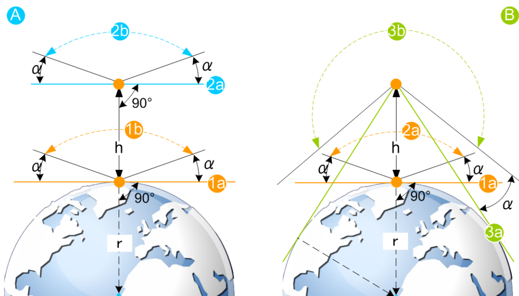
Figure 6-2: Impact of the Earth Obscuration Reference on the area of visible satellites (XY cut)
