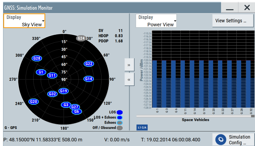
Figure 8-6: Monitoring effects of static multipath configuration for GPS space vehicles
