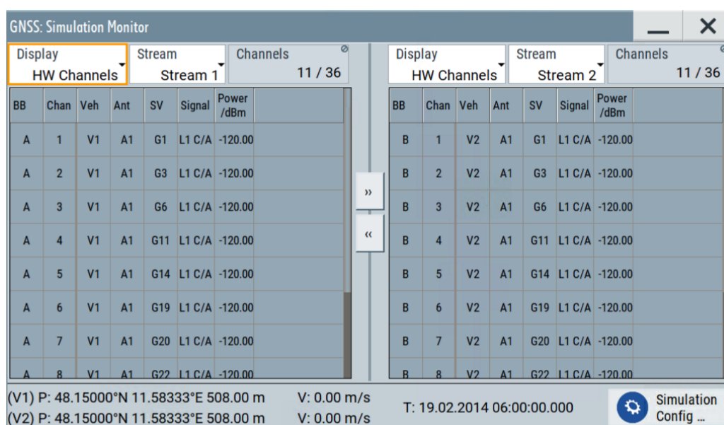
Figure 15-1: HW channels view for GNSS Stream 1 and GNSS Stream 2
