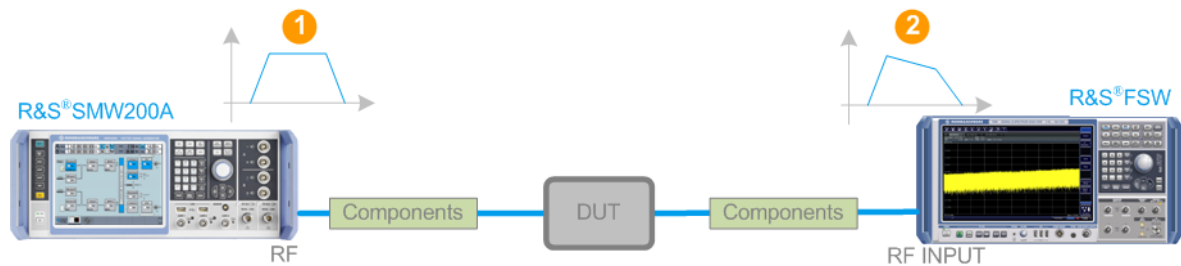
Figure 2-1: Effect of the non-linear frequency response in the components on the signal flatness
