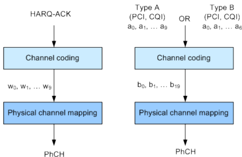
Figure 2-9: Channel coding for HS-DPCCH (MIMO mode)
