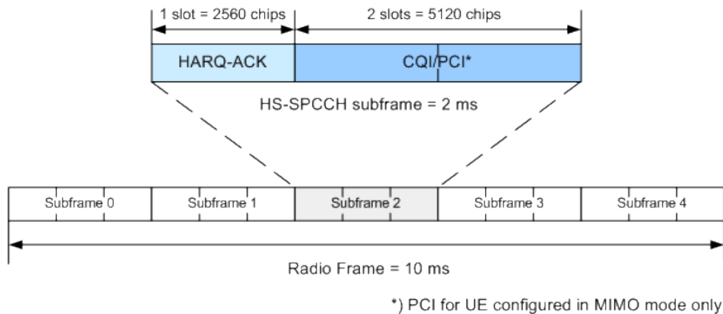
Figure 3-18: Structure of an uplink HS-DPCCH in the time domain
