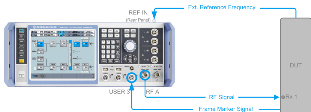
Figure 5-1: Test Setup
