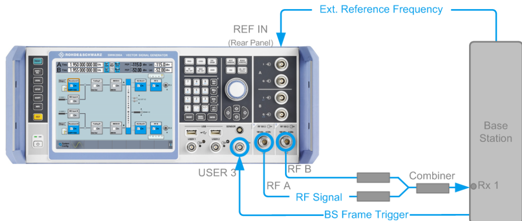
Figure 6-2: Standard Test Setup (Two Paths)
