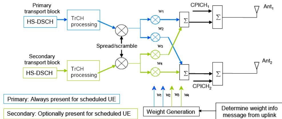
Figure 2-8: MIMO for HSPA+
