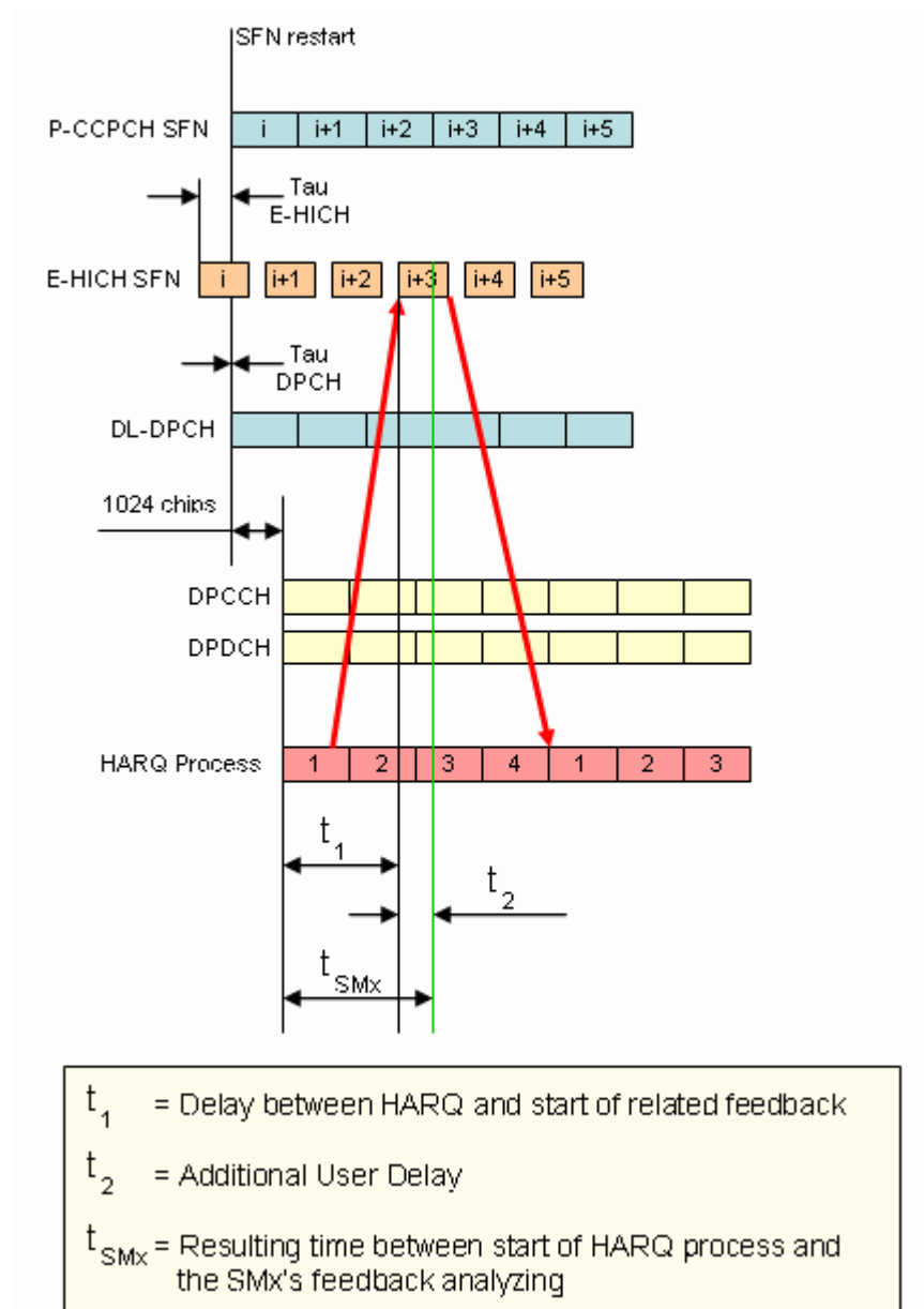
Figure 2-7: Timing diagram for TTI 10ms, \tau_{dpch} = 0 , \tau_{E-HICH} = -7\text{slots}
