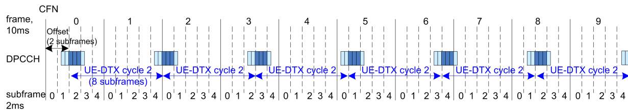
Figure 4-1: Example for UL DPCCH DTX burst pattern as generated by the R&S SMW (E-DCH TTI=2ms, beginning at CFN0, UE_DTX_DRX_Offset=2, DTX Cycle 2=8 subframes)
