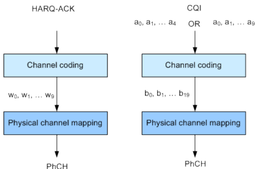
Figure 2-12: Channel coding for HS-DPCCH (non-MIMO mode)
