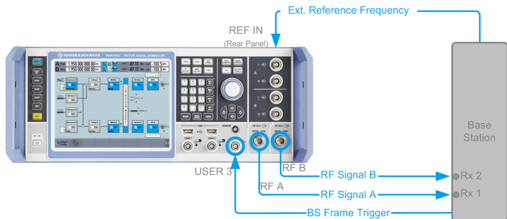
Figure 6-3: Standard Test Setup (Diversity Measurements)
