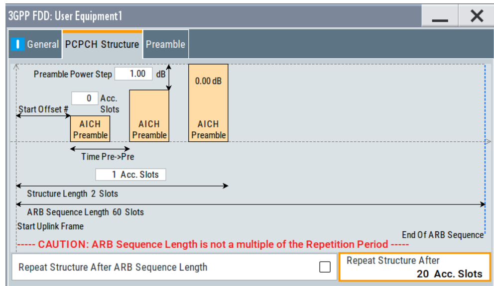
Figure 3-29: PCPCH Structure in "Mode > PCPCH preamble-only"
