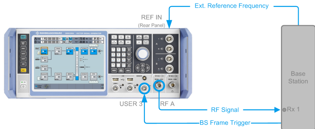
Figure 6-1: Standard Test Setup (One Path)
