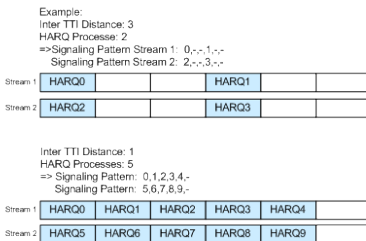
Figure 3-9: Example: Inter TTI Distance in HSDPA H-Set Mode
