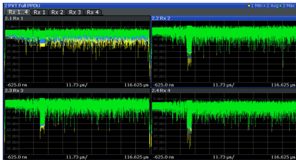
Figure 3-22: PVT Full PPDU result display for IEEE 802.11n MIMO measurements
