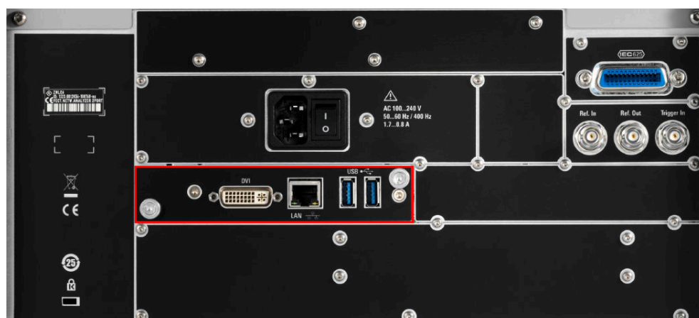
Figure 5-1: Location of the PC board for R&S FPL1000
