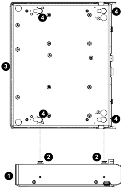
Figure 3-7: Aligning R&S TSMA6B-BP and R&S TSMA6/6B
