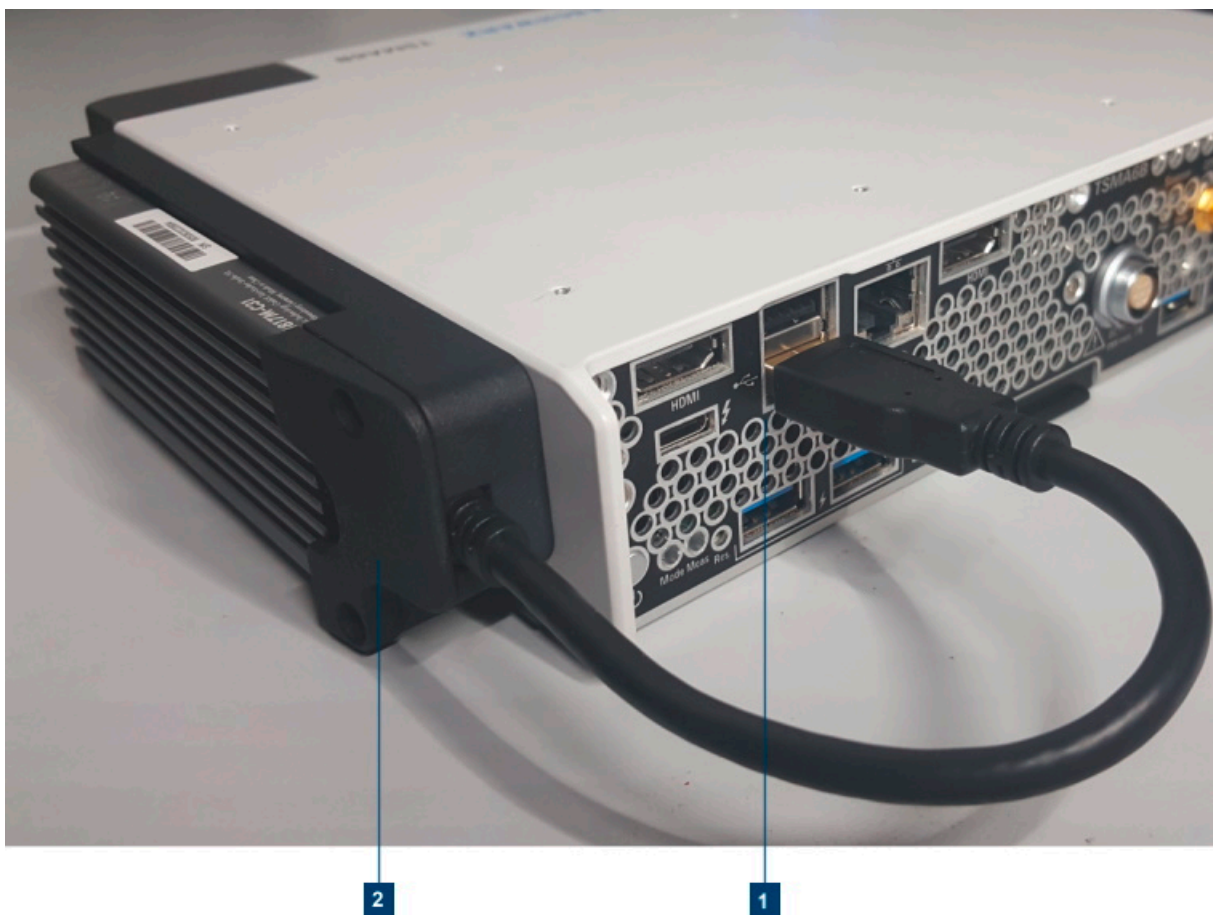
Figure 3-2: R&S TSMA6B - removable disk option
