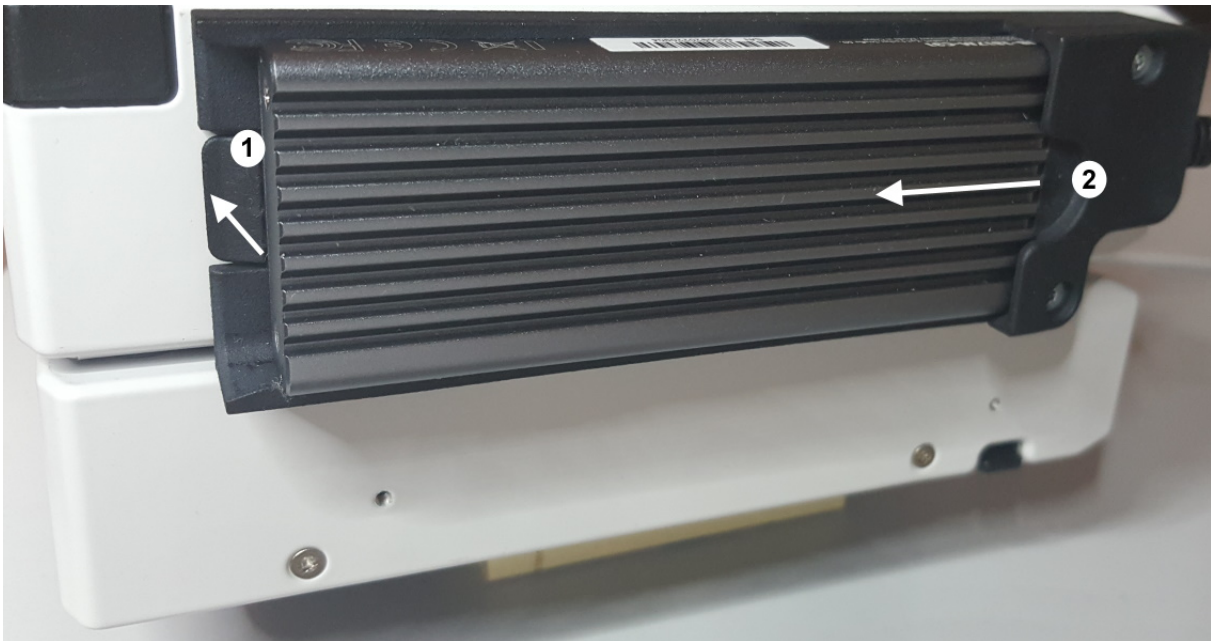
Figure 3-3: Remove SSD enclosure
