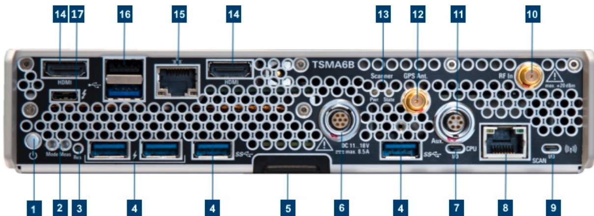
Figure 4-2: R&S TSM6B - Rear Panel
