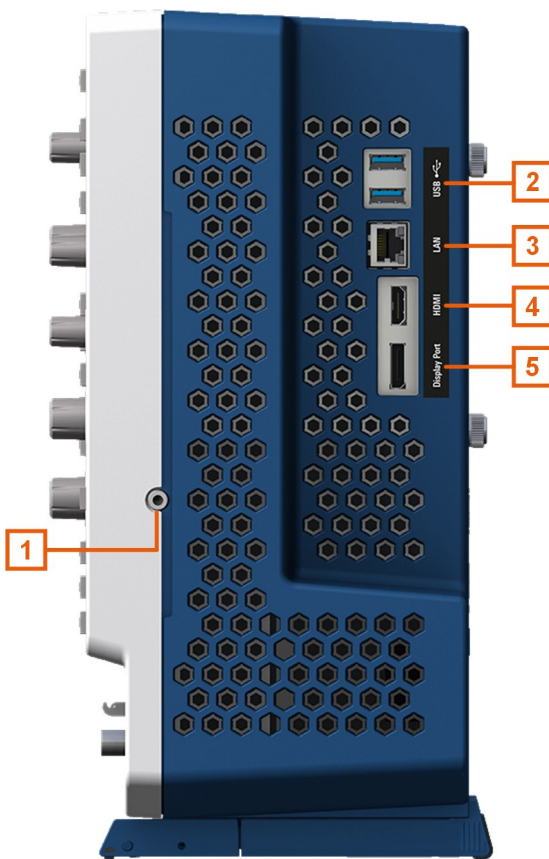
Figure 5-2: Side view of R&S MXO 5
