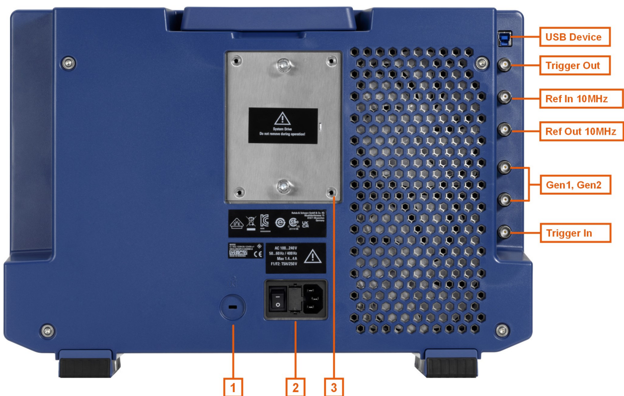
Figure 5-3: Rear panel view of R&S MXO 5
