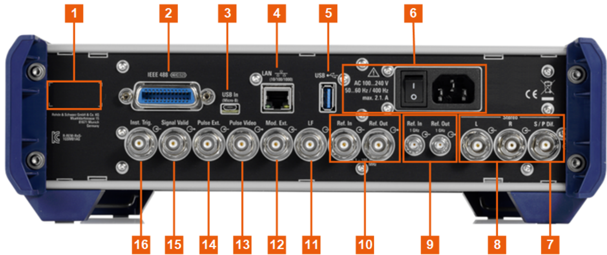
Figure 5-4: Rear panel view R&S SMB100B RF signal generator
