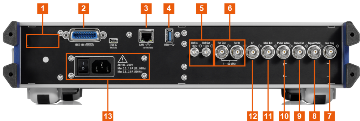
Figure 5-5: Rear panel view R&S SMB100B Microwave signal generator
