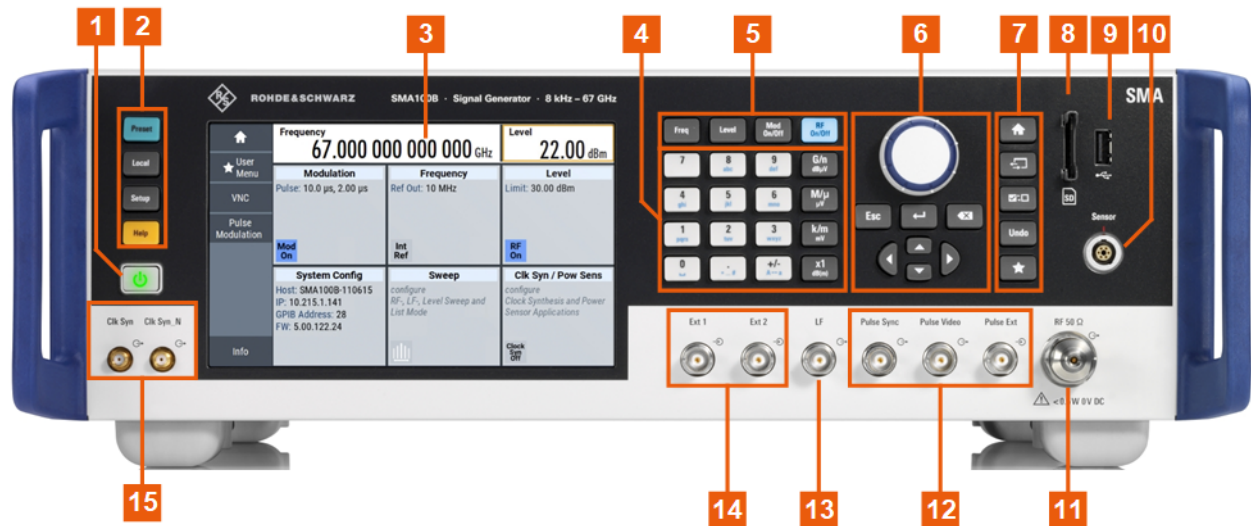
Figure 5-2: Front panel view of R&S SMA100B (3 HU, R&S SMAB-B93)
