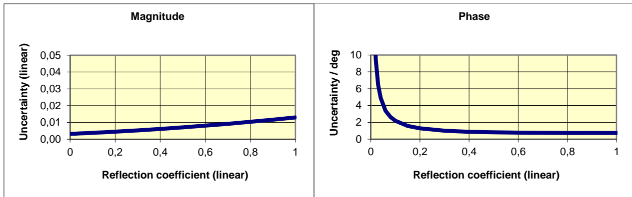
Typical accuracy of reflection magnitude and reflection phase measurements of the R&S®ZVA8 in the frequency range 1 MHz to 8 GHz, of the R&S®ZVA24 in the frequency range 50 MHz to 24 GHz, of the R&S®ZVA40 in the frequency range 50 MHz to 40 GHz, of the R&S®ZVA50 in the frequency range 50 MHz to 50 GHz and of the R&S®ZVA67 in the frequency range 50 MHz to 67 GHz
