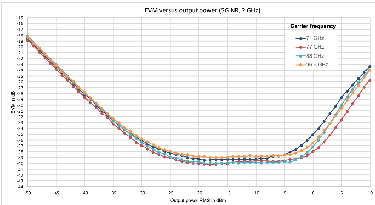
EVM values versus output power at different center frequencies with R&S®SMW200A (with R&S®SMW-B711 option) in combination with R&S®FE110SR and R&S®FSW (with R&S®FSW-B4001 option), IF mode: EVM optimized
