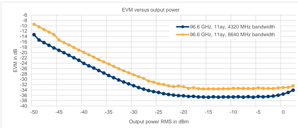
EVM values versus output power with R&S®SFI100A in combination with R&S®FE110SR and R&S®FSW (with R&S®FSW-B8001 option), IF mode: EVM optimized
