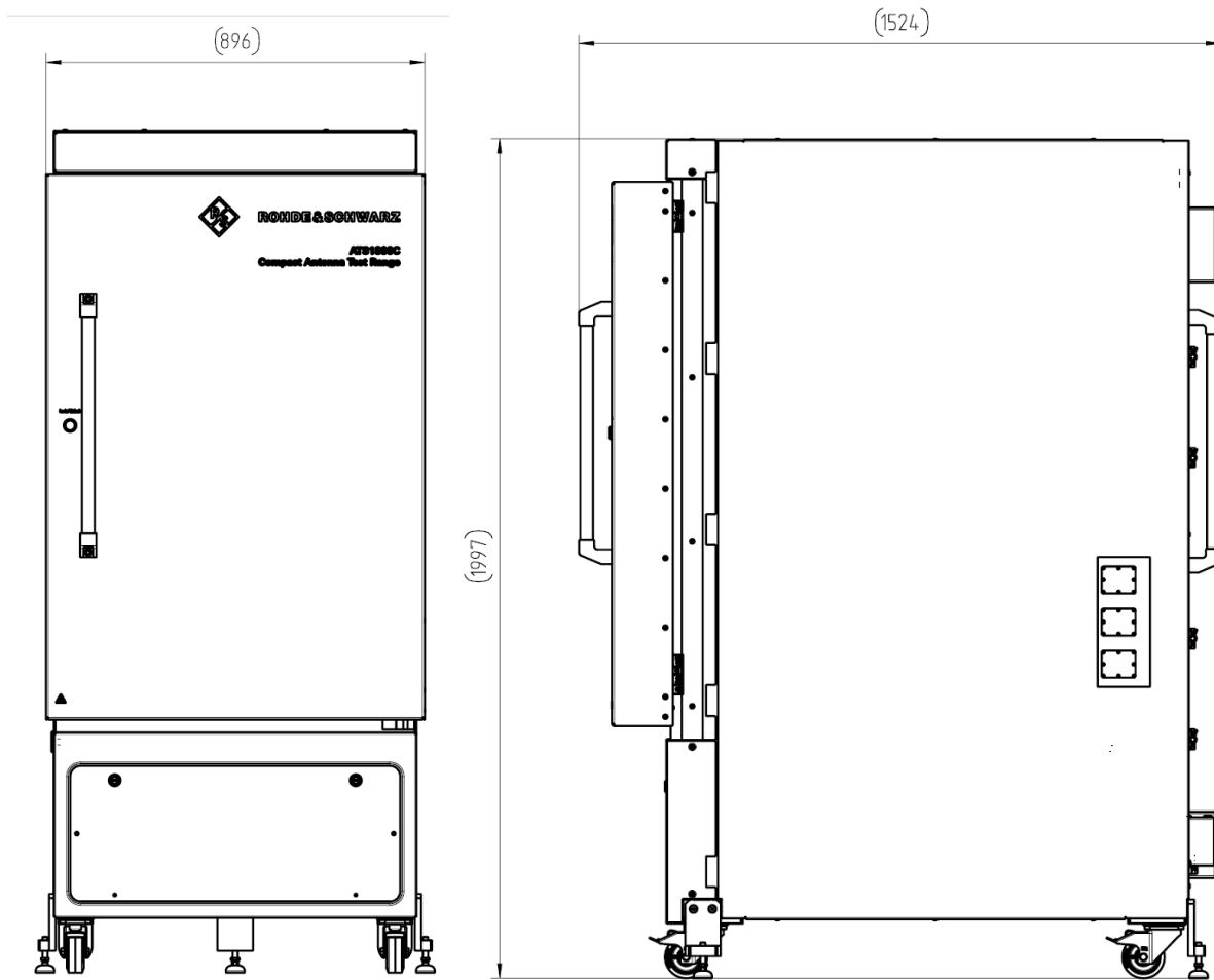
R&S®ATS1800C: front and side view
