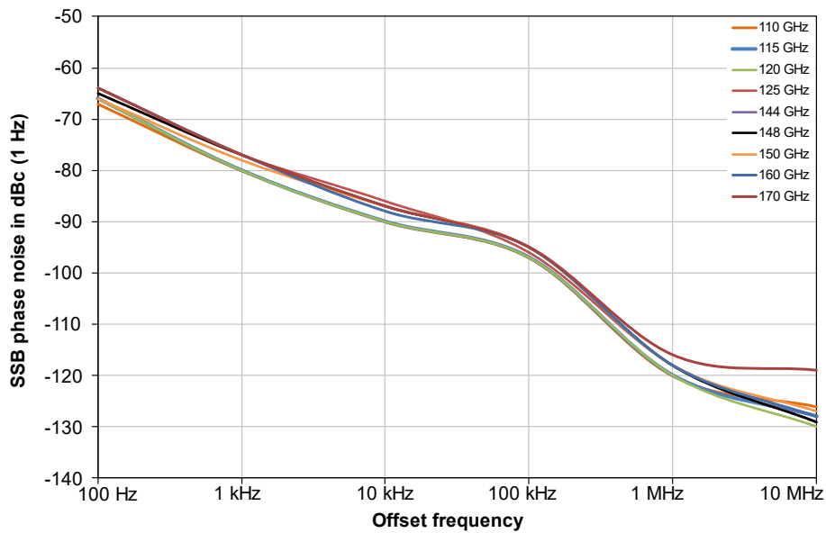
Measured single sideband phase noise in combination with an R&S®FE170ST
