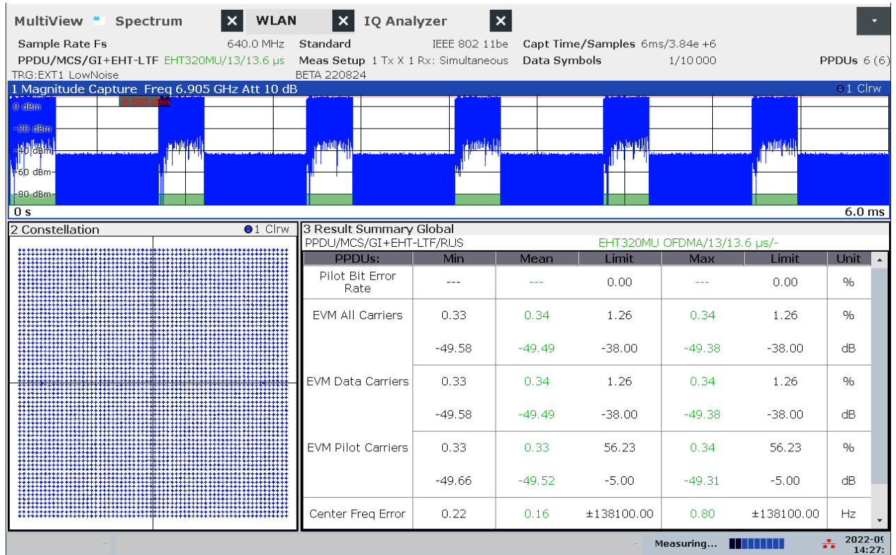
Measured EVM for an IEEE 802.11be signal with 320 MHz bandwidth
