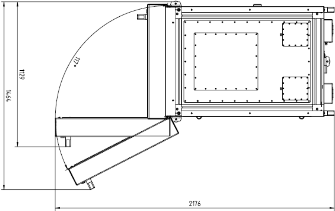
R&S®ATS1500C: top view
