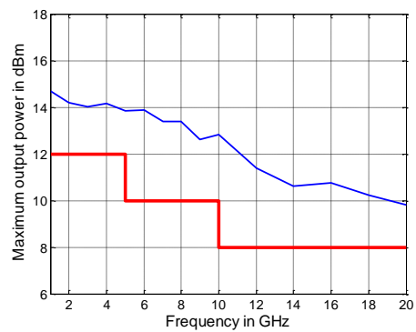
Measured maximum output power in dBm versus frequency for the R&S®ZNBT20
