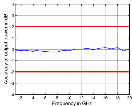
Measured output power accuracy in dB versus frequency for the R&S®ZNBT20
