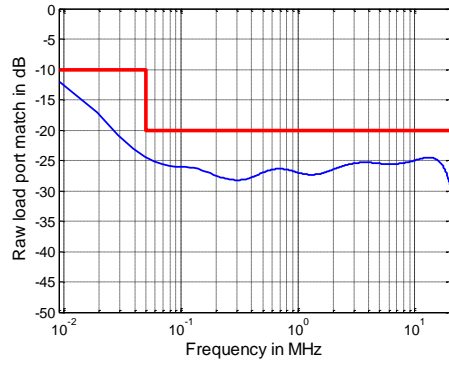
Measured raw load port match versus frequency for the R&S®ZNBT8
