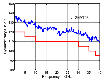
Measured dynamic range in dB versus frequency for the R&S®ZNBT26/R&S®ZNBT40
