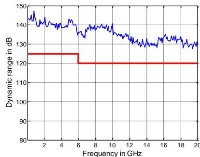
Measured dynamic range in dB versus frequency for the R&S®ZNB T20
