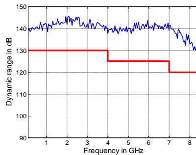
Measured dynamic range in dB versus frequency for the R&S®ZNB T8
