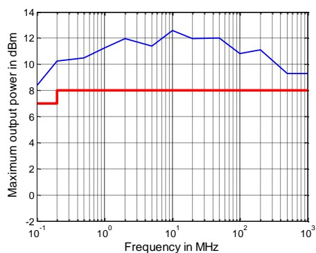
Measured maximum output power in dBm versus frequency for the R&S®ZNBT26 and R&S®ZNBT40
