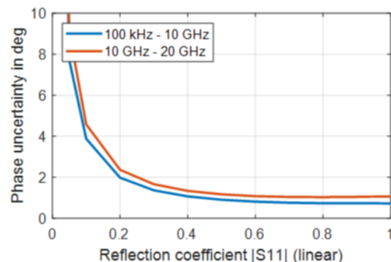
Uncertainty of reflection magnitude and reflection phase measurements for the R&S®ZNB20 in the frequency range from 100 kHz to 20 GHz; analysis conditions: S_{12} = S_{21} = 0 , calibrated power –10 dBm, measured power –10 dBm
