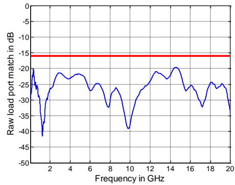
Measured raw load port match versus frequency for the R&S®ZNBT20
