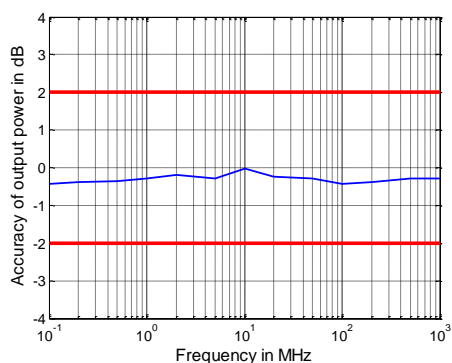
Measured output power accuracy in dB versus frequency for the R&S®ZNBT26 and R&S®ZNBT40
