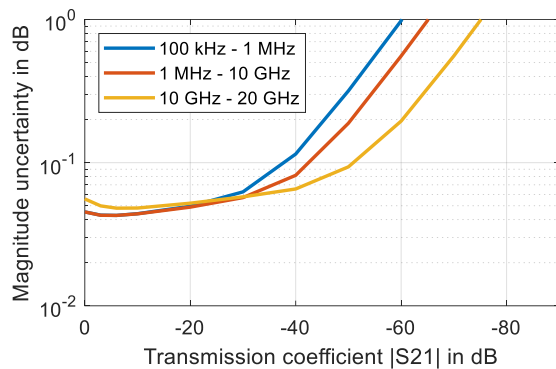
Uncertainty of transmission magnitude and transmission phase measurements for the R&S®ZNB20 in the frequency range from 100 kHz to 20 GHz; analysis conditions: S_{11} = S_{22} = 0 , calibrated power –10 dBm, measured power –10 dBm
