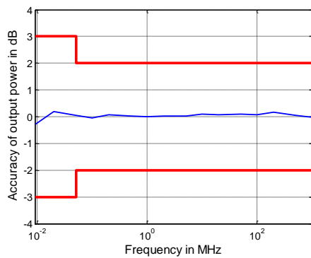
Measured output power accuracy in dB versus frequency for the R&S®ZNBT8
