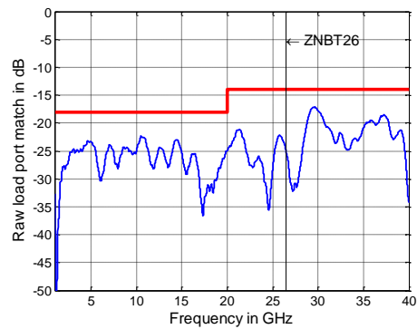
Measured raw load port match versus frequency for the R&S®ZNBT26 and R&S®ZNBT40
