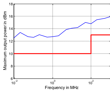
Measured maximum output power in dBm versus frequency for the R&S®ZNBT8
