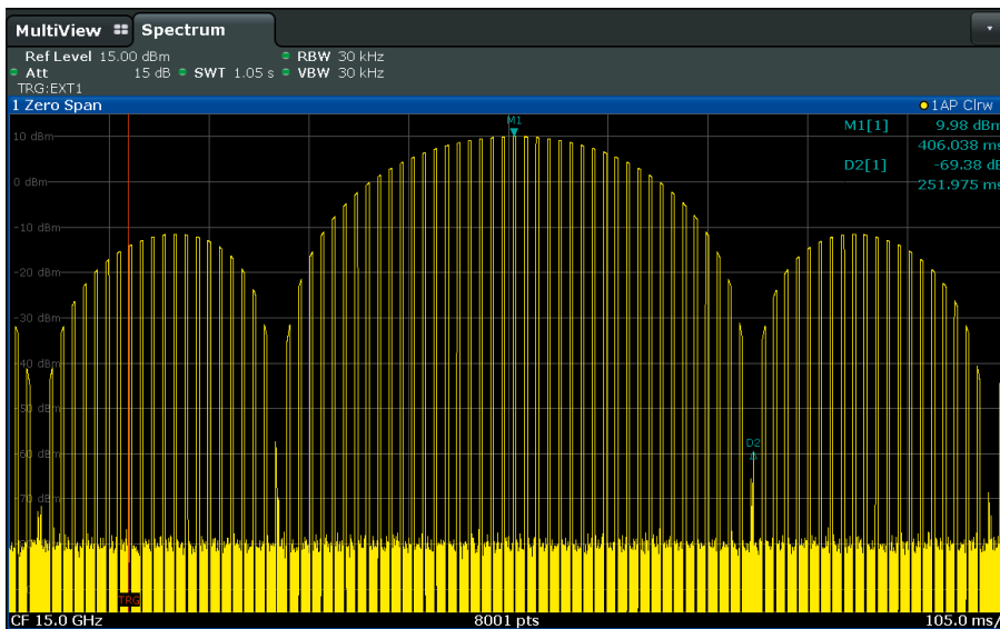
Pulse and amplitude-modulated signal generated with the R&S®SMA100B. The \sin(x)/x modulation signal is fed at the external analog modulation input and used to produce a signal with 70 dB (meas.) modulation depth.
