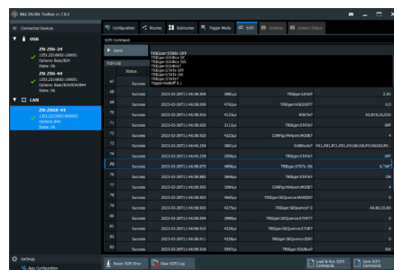
Command and control using SCPI, including switch matrix feedback logs
