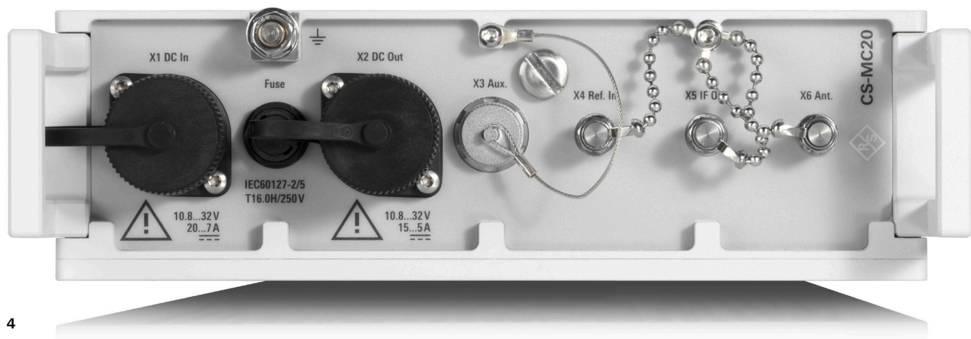
R&S®CS-MC20 microwave converter
