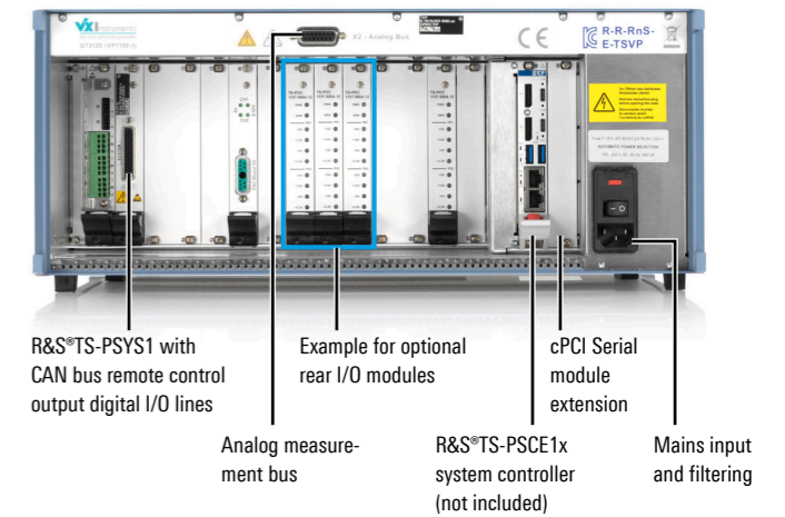
R&S® ExpressTSVP rear view
