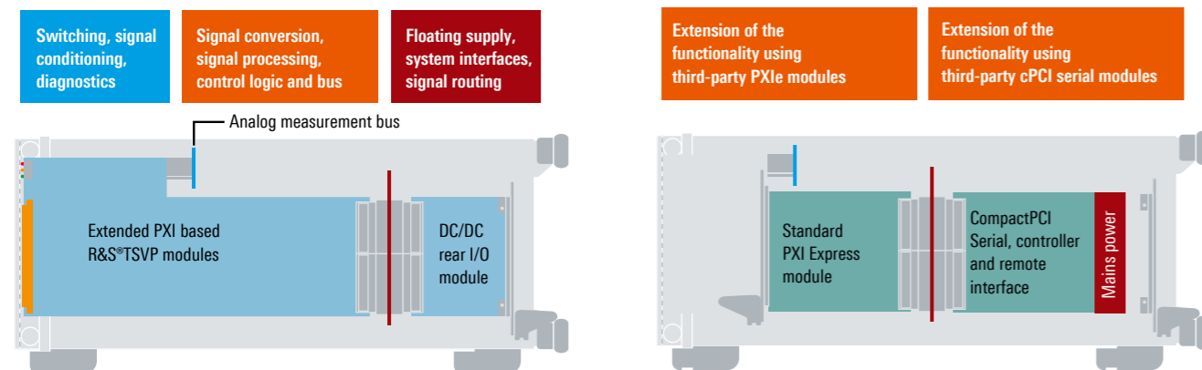
Slots S3 to S16: Rohde & Schwarz extended modules
