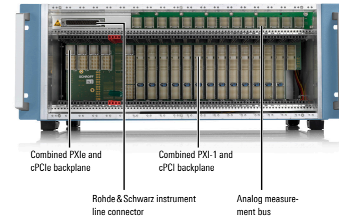
R&S® ExpressTSVP front view
