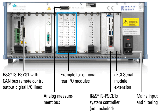
R&S® ExpressTSVP rear view
