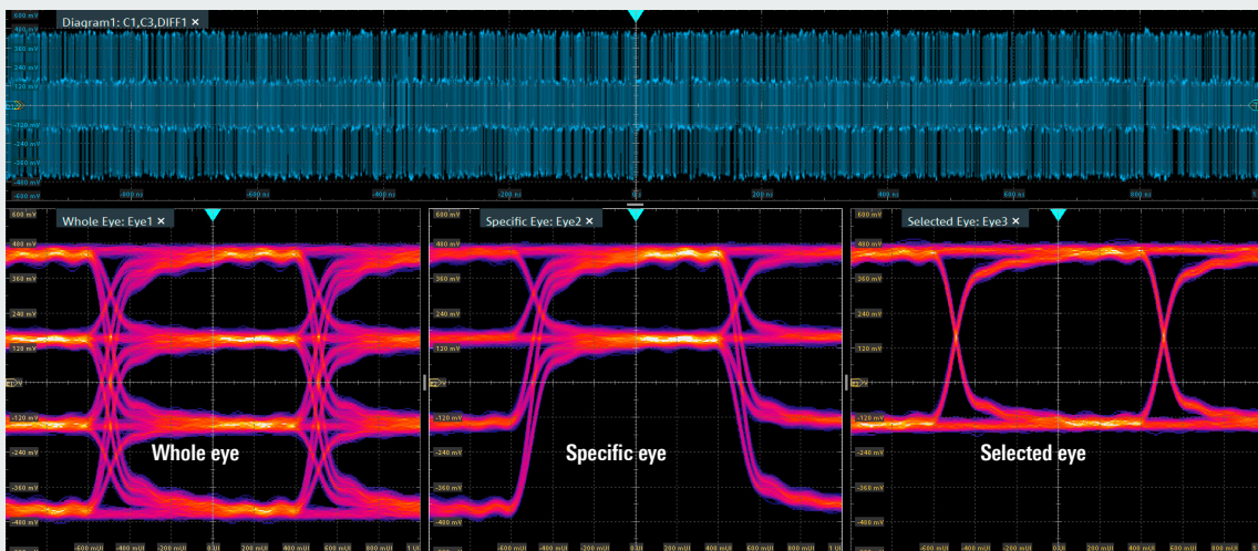
PAM-3 signal analysis: Eye diagram display with whole, selected and specific filter mode
