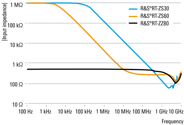
Input impedance versus frequency
