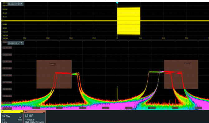
Direct acquisition and analysis of sporadically occurring EMI thanks to the R&S®RTO6 oscilloscope's powerful spectrum analysis function
