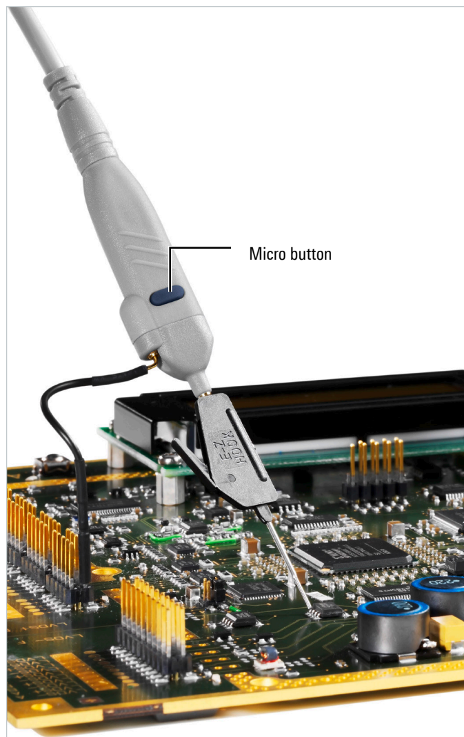
Practical design: micro button for convenient instrument control Diverse probe tips and ground cables are included as standard.
