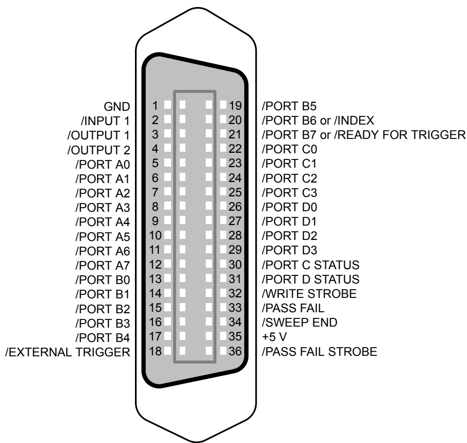
Figure 2-1: Pin Assignment of the Handler I/O Connector
