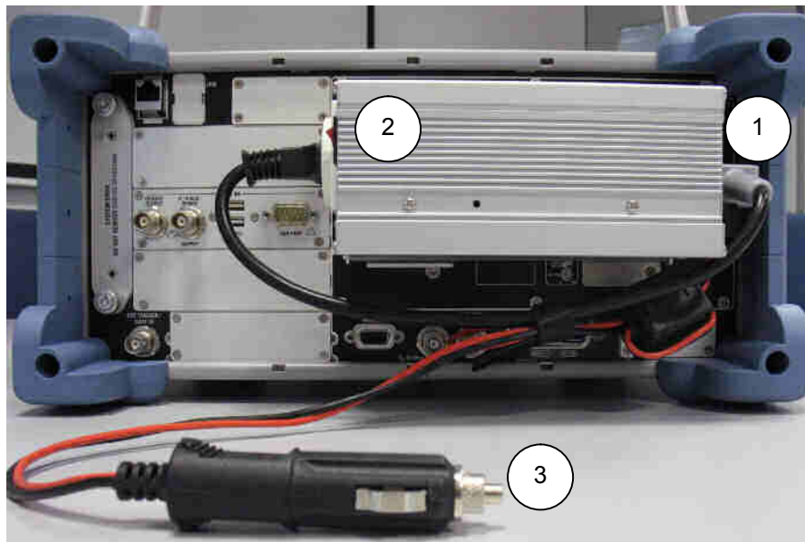
Figure 1-2: Rear panel view of the R&S FSV
