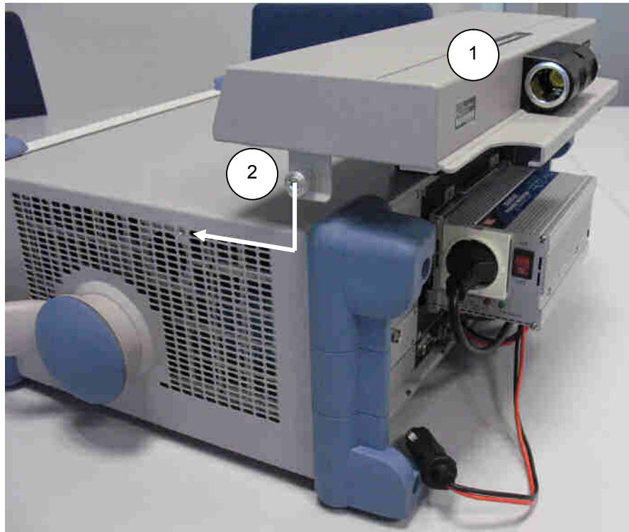
Figure 2-1: Installation of the battery pack
