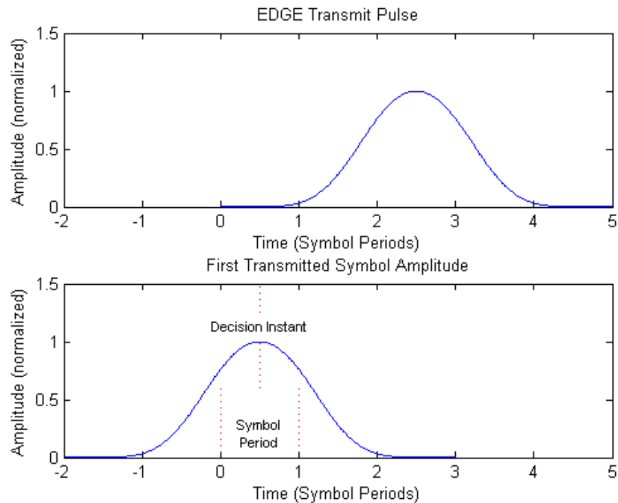
Figure 3-30: EDGE transmit pulse (top) and the first transmitted symbol (bottom)
