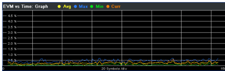
Figure 3-4: EVM vs Time graph
