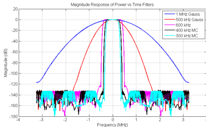
Figure 3-26: Magnitude Response of the Power vs Time Filters
