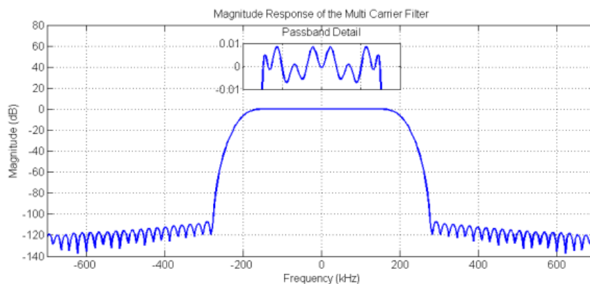
Figure 3-25: Frequency Response of the Multi Carrier Filter
