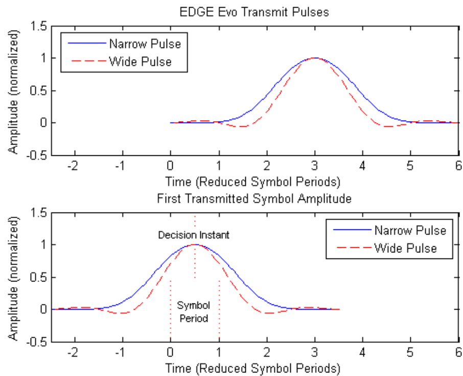
Figure 3-31: EDGE Evolution transmit pulses (top) and the first transmitted symbols (bottom)
