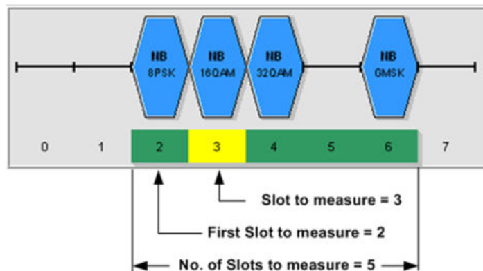
Figure 3-23: Concept of "First Slot to measure", "Number of Slots to measure" and "Slot to Measure"
