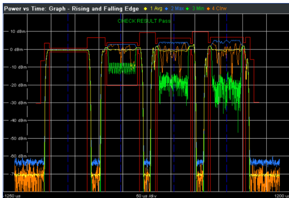
Figure 3-11: Rising and Falling Edge view in Power vs Time
