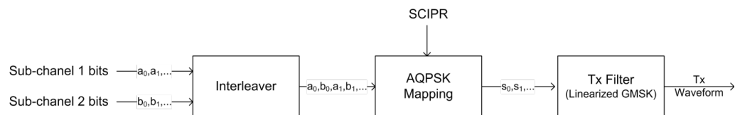
Figure 3-21: AQPSK modulation scheme for GSM systems
