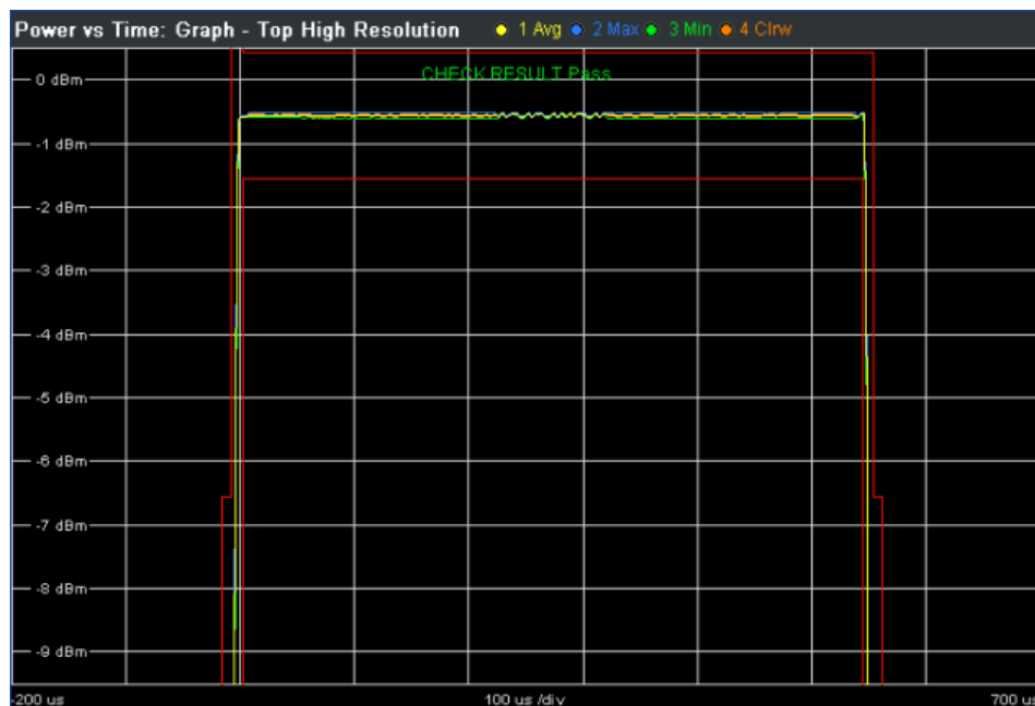
Figure 3-12: Top High Resolution view in Power vs Time
