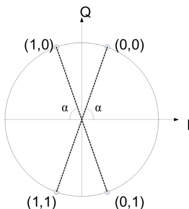
Figure 3-22: AQPSK constellation [reproduced from 3GPP change request document GP-100275].
