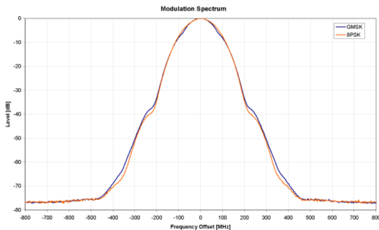
Figure 3-20: GMSK and 8PSK modulation spectrum
