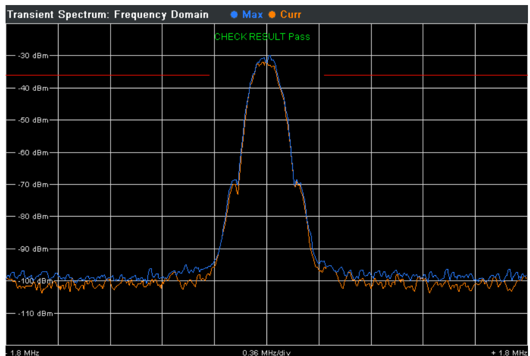
Figure 3-16: Frequency Domain of Transient Spectrum with traces and limits (red)
