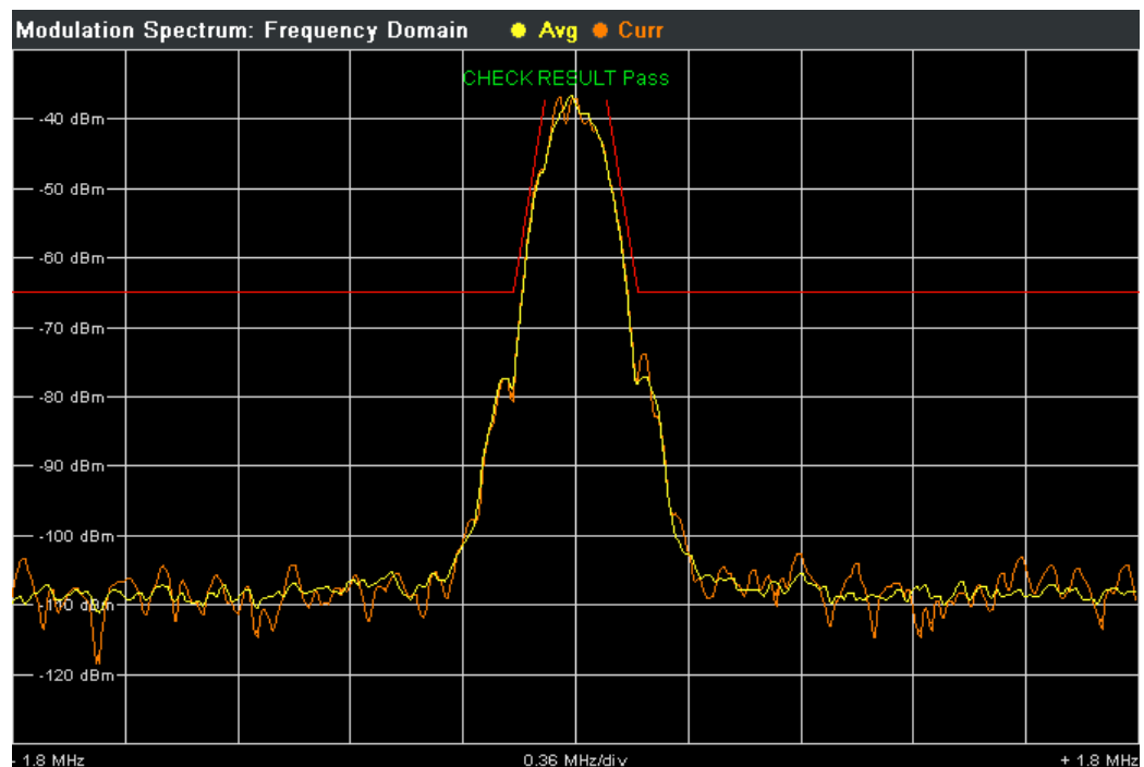
Figure 3-14: Frequency Domain of modulation spectrum with traces and limits (red)
