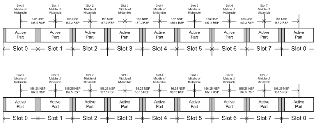
Figure 3-34: "Not equal"(top) and "equal" (bottom) timeslot length criteria
