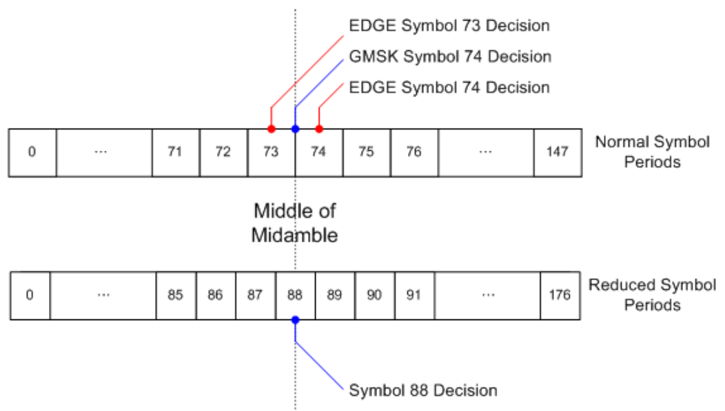
Figure 3-33: Middle of midamble for normal and reduced symbol period bursts.
