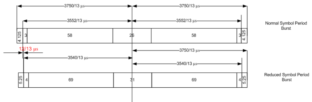
Figure 3-32: Timing alignment between normal symbol period and reduced symbol period bursts
