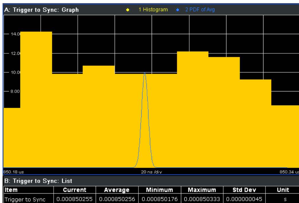
Figure 3-9: Trigger to Sync
