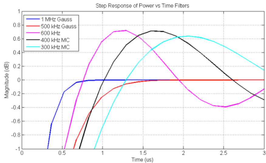
Figure 3-27: Step Response of the Power vs Time Filters
