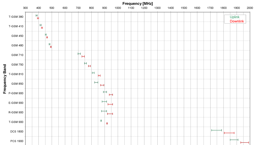
Figure 3-19: The frequencies specified in the GSM standard
