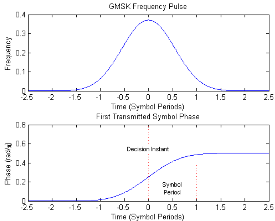
Figure 3-29: GMSK Frequency Pulse (top) and phase of the first tail symbol (bottom)
