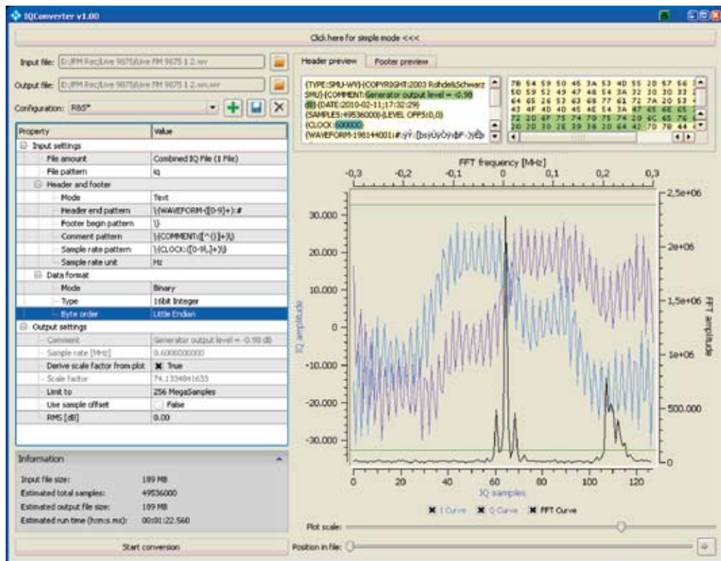
I/Q converter tool.
