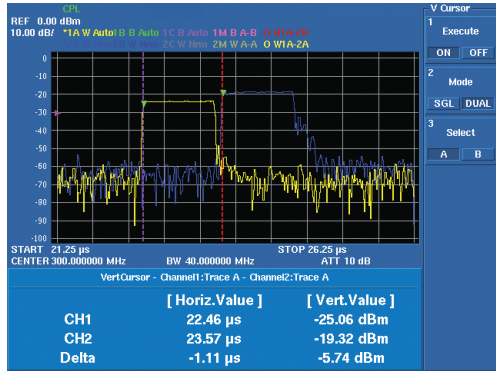
Overlay display: Power vs. time comparison of two signals
