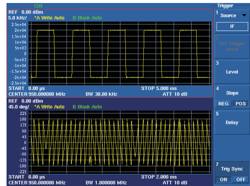
Frequency vs. time analysis
