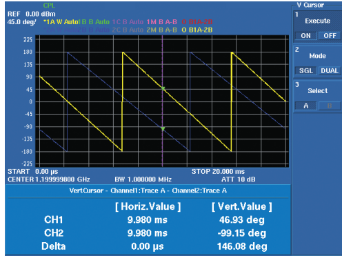
Overlay display: Phase vs. time comparison of two signals
