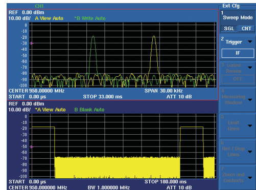
FFT analysis
