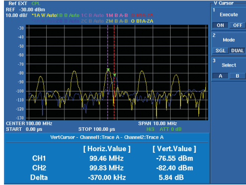
Overlay display: FFT comparison of two signals
