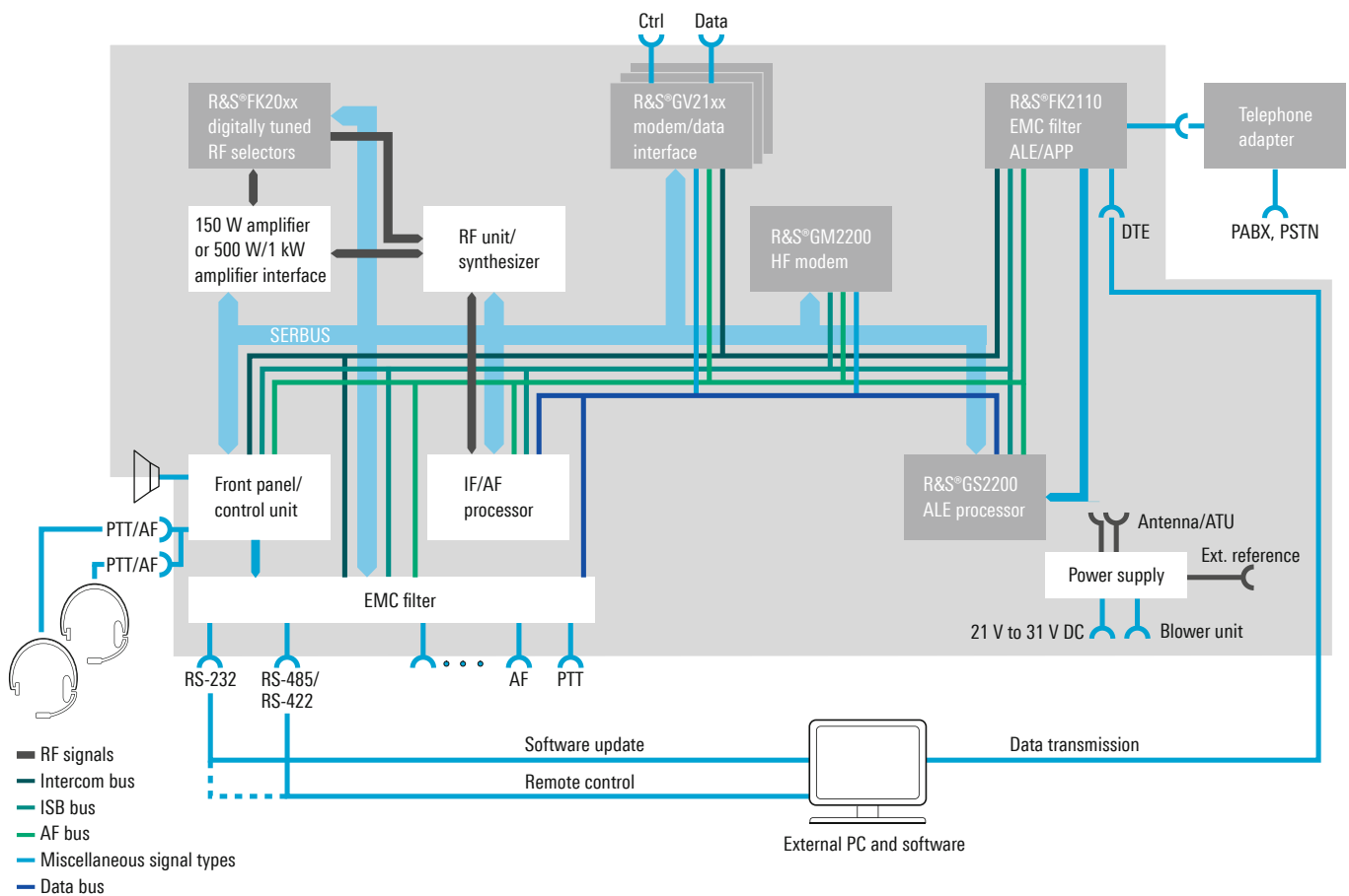
Block diagram of the R&S®XK2100 and R&S®GX2900
