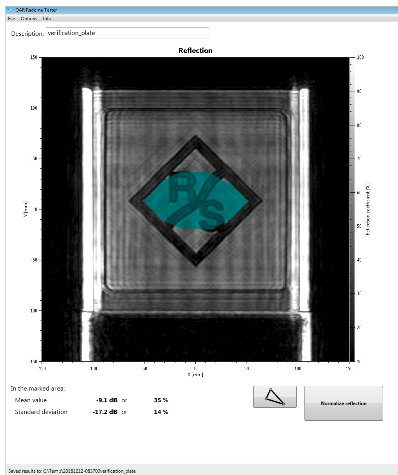
Resulting image of a high-resolution reflectivity measurement of a Rohde & Schwarz radome with 500 µm thickness mismatch
