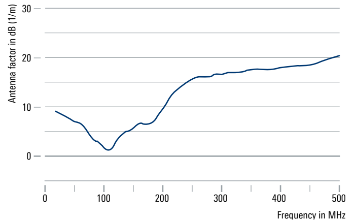
Typical antenna factor
