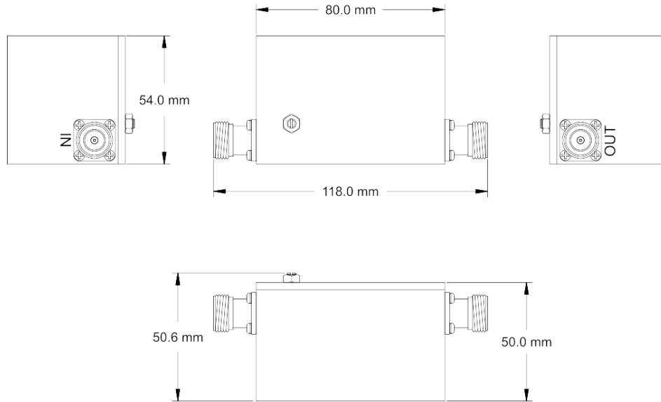
Indoor Passband Filter Outline Drawing BPT-0832862-0-S3
