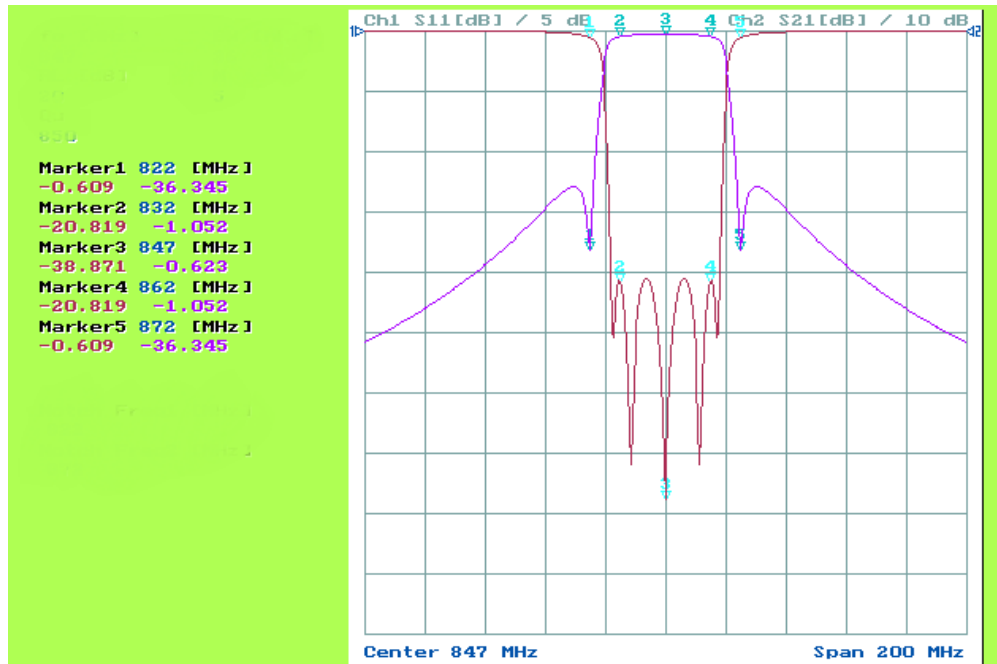
BPT-0832862-0-S3 RX Filter Characteristics
