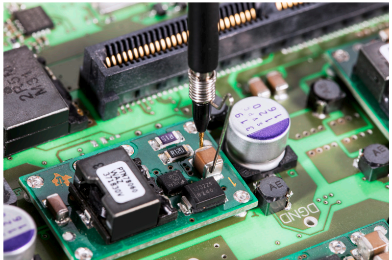
The R&S®RT-ZPR20 probe's browser extension is the perfect tool for verifying the DC levels of multiple power supplies on a PCB.
