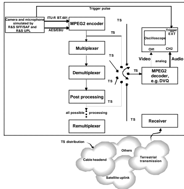
Fig 5 The audio-to-video delay measurement scenario.
