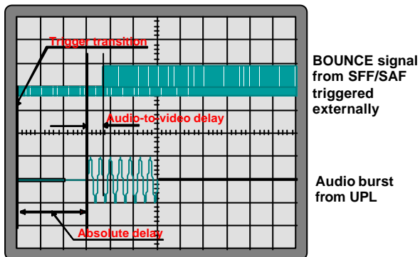
Fig 6 Oscilloscope display for measurement of absolute delay and audio-to-video delay.
