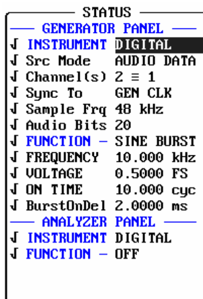
Fig 1 Settings in R&S UPL.
