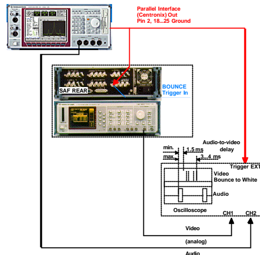
Fig 3 Compensating for overall delay.
