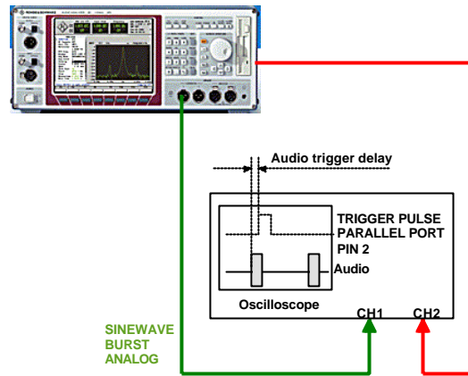
Fig 2 R&S UPL time offset between trigger pulse and sine burst without compensation.
