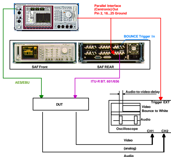
Fig 4 Measurement setup for audio-to-video delay.
