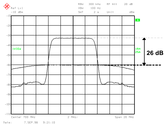
Fig. 9 PRBS useful signal and noise spectra with 10 dB/div
