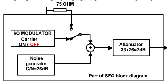
Fig. 8 CODER switched off by firmware and noise path in SFQ
