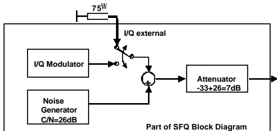
Fig. 7 Useful signal and noise paths in SFQ
