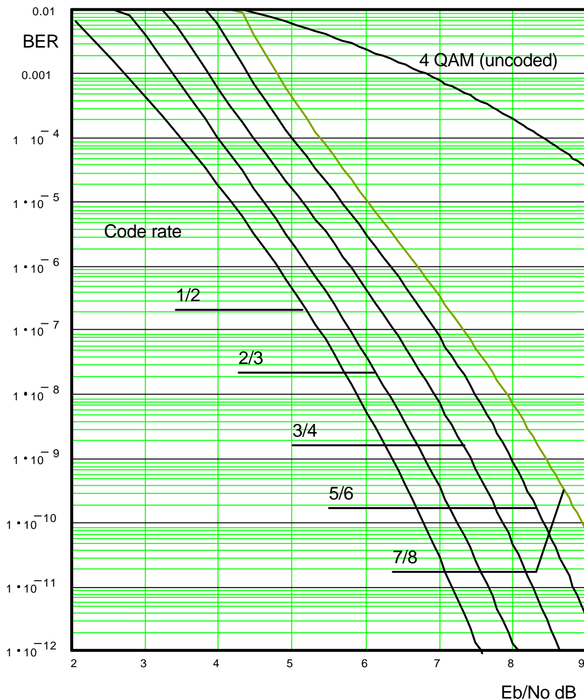
Fig. 13 BER as a function of E_b/N_0
