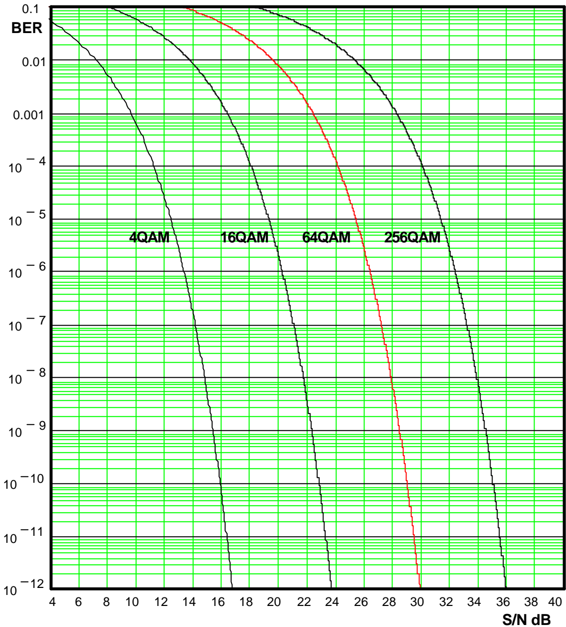
Fig. 10 BER as a function of S/N
