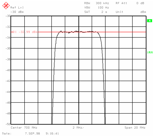
Fig. 6b PRBS spectrum: level marked with display line, 1 dB/div for highest precision
