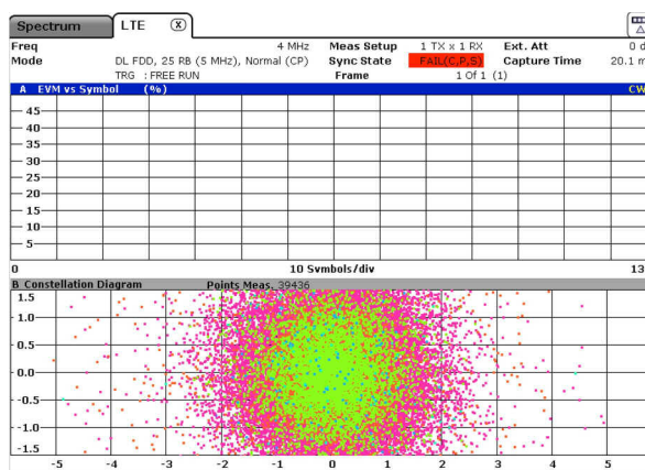
Figure 2-9: Attempt to demodulate a low SNR LTE signal in the presence of strong adjacent interference signal
