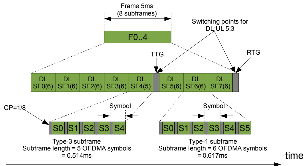
Figure 11: TDD frame structure of 802.16m for 5, 10 and 20 MHz
