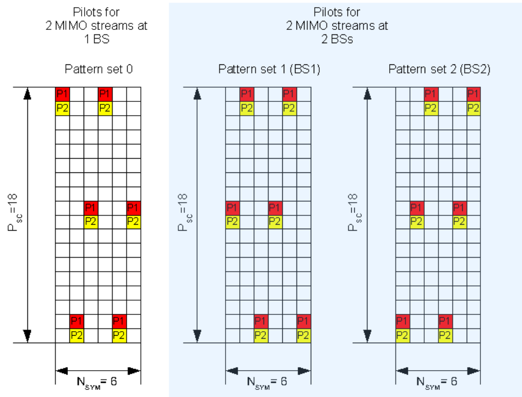
Figure 17: DL pilot pattern for 1 and 2 transmission streams
