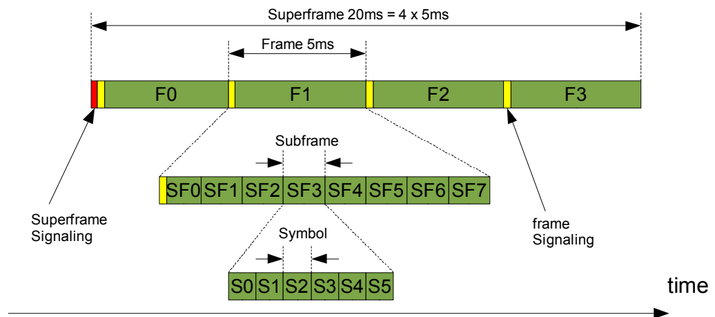
Figure 9: superframe structure in 802.16m
