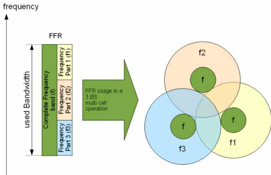
Figure 15: multi cell operation with FFR
