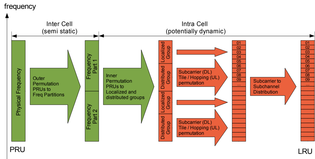
Figure 16: PRU to LRU mapping (DL, UL)
