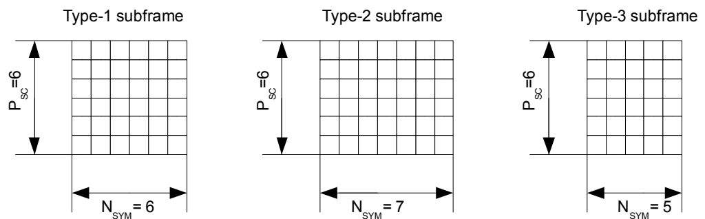
Figure 14: UL physical resource unit partitions
