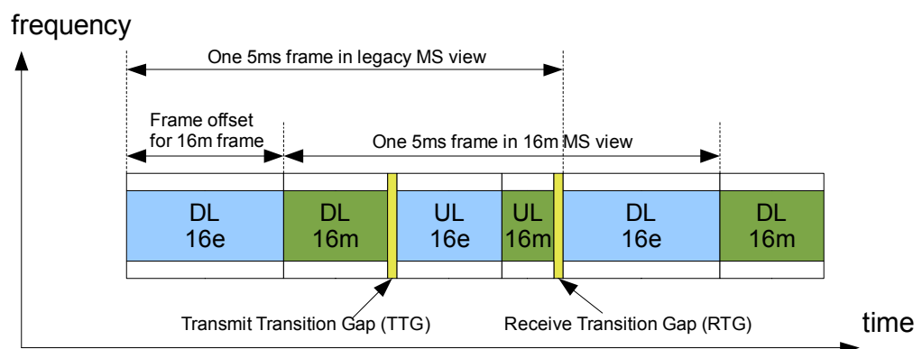
Figure 6: legacy support in 802.16m
