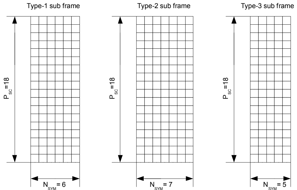
Figure 12: DL and UL physical resource unit
