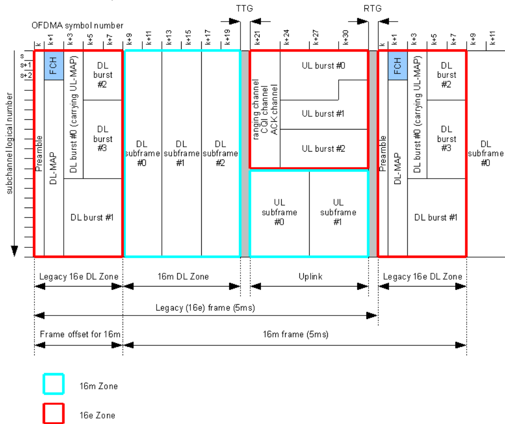
Figure 8: 802.16m TDD legacy frame with FDM UL
