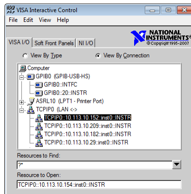
Figure 2: VISA Interactive Control program
