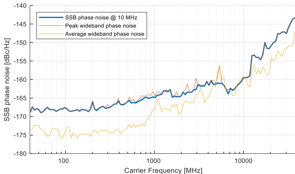
Figure 15 R&S®SMA100B (with B711) wideband phase noise (meas.)
