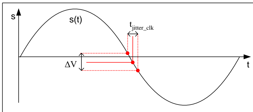
Figure 5 Voltage error \Delta V due to jitter on the sampling clock t_{\text{jitter,clk}}
