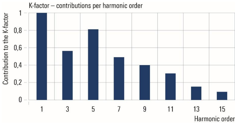
Figure 21: Diagram of the contributions per harmonic to the K-factor of approx. 3.8
