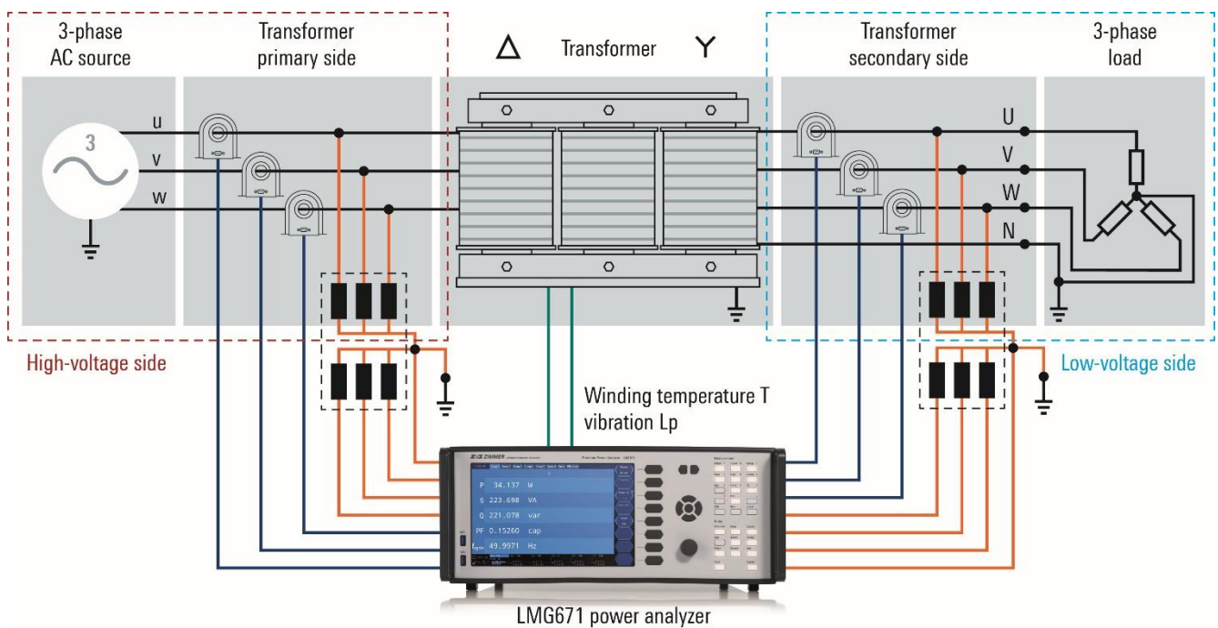
Figure 9: Transformer efficiency test and connection to the LMG671 power analyzer
