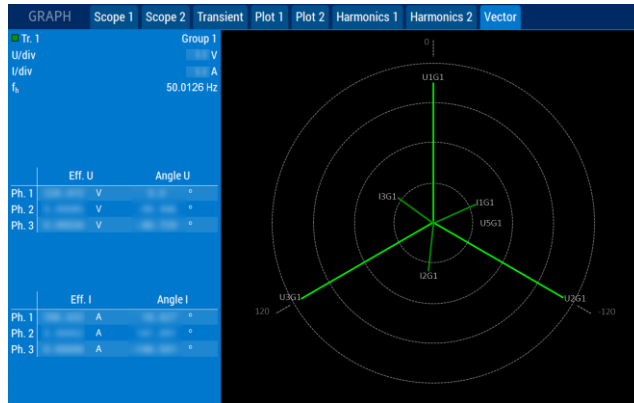
Figure 13: Vector diagram - extract from LMG671 Scope menu for checking phase symmetry
