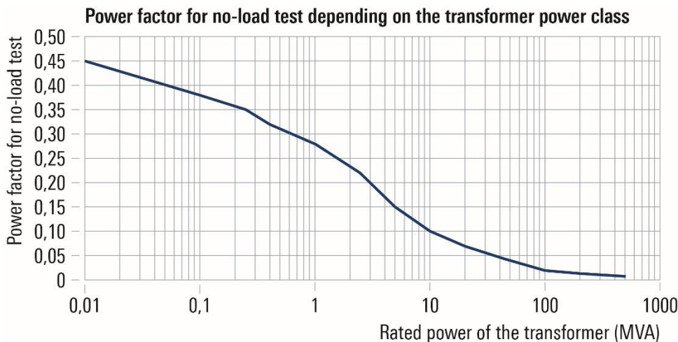
Figure 4: Power factors for no-load tests as a function of the transformer power class
