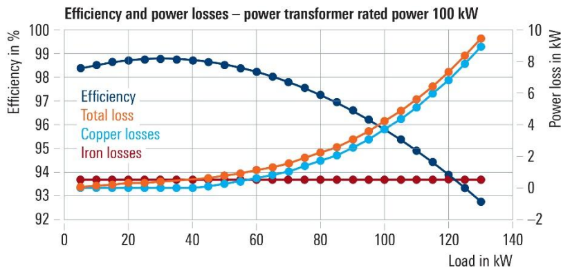
Figure 11: Typical efficiency curve of a transformer
