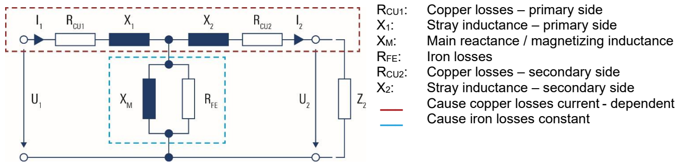
Figure 1: Simplified equivalent circuit of a loaded transformer
