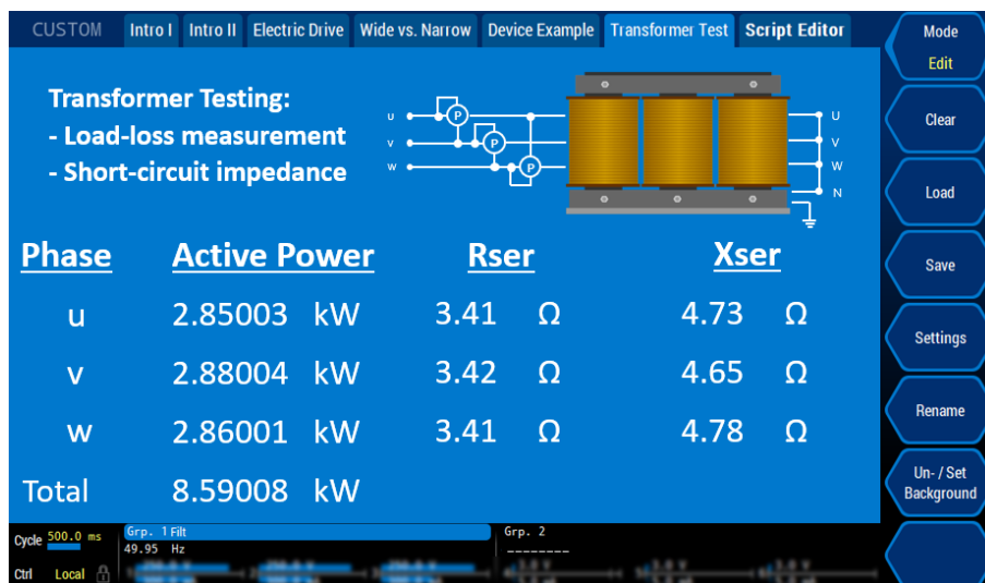
Figure 8: Exemplary LMG671 "Custom Menu" for the short-circuit test
