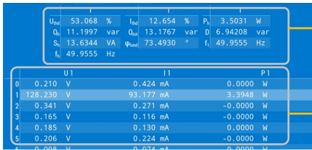
Figure 12: LMG671 example display of measured harmonic values
