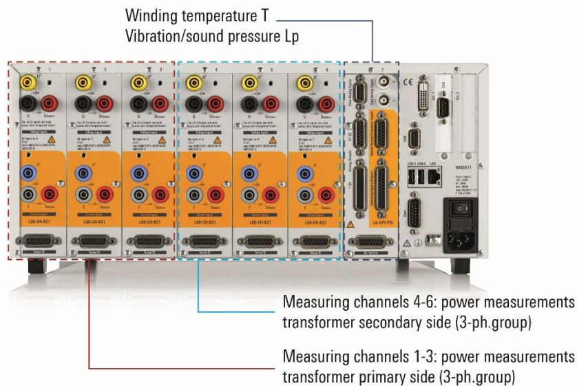
Figure 10: Connection of transformer primary and secondary side to the LMG671 power analyzer
