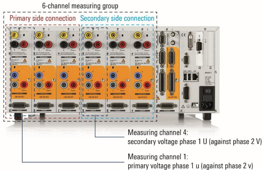
Figure 15: Connection and grouping of measuring solution 1 for testing the phase displacement
