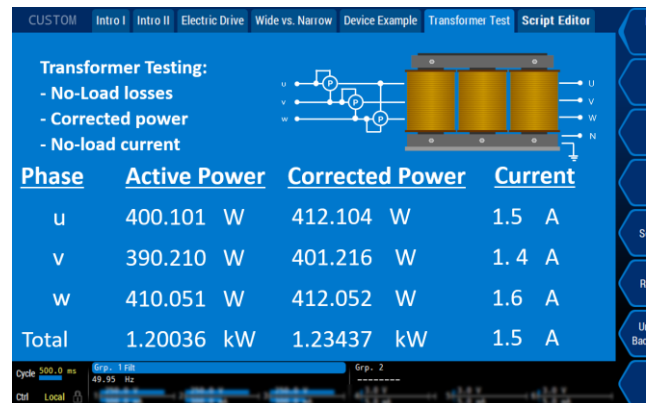
Figure 6: Exemplary LMG671 "Custom Menu" for the no-load test
