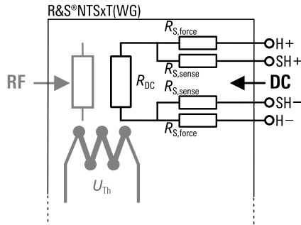
Figure 18 Parasitic series resistances in DC heater supply lines of R&S®NTS
