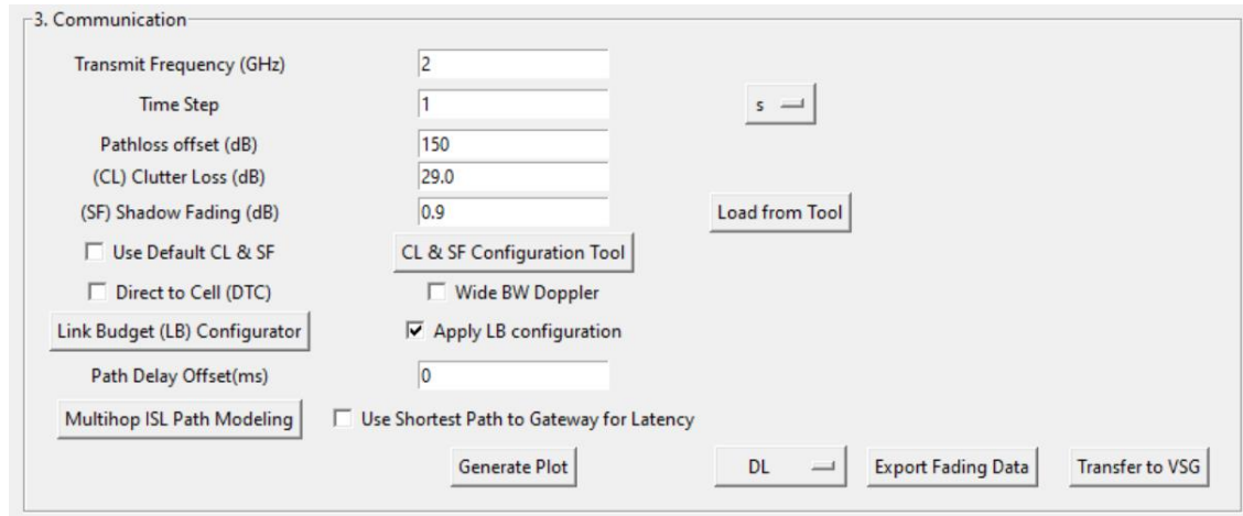
Figure 10: Communication section of the R&S Space Nexus
