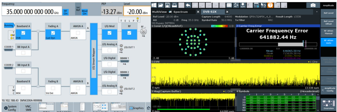
Figure 21: Simulation Example on SMW200A and FSW
