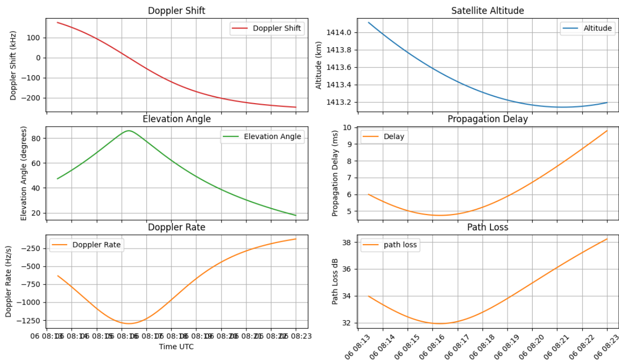
Figure 11: Propagation parameter plot example
