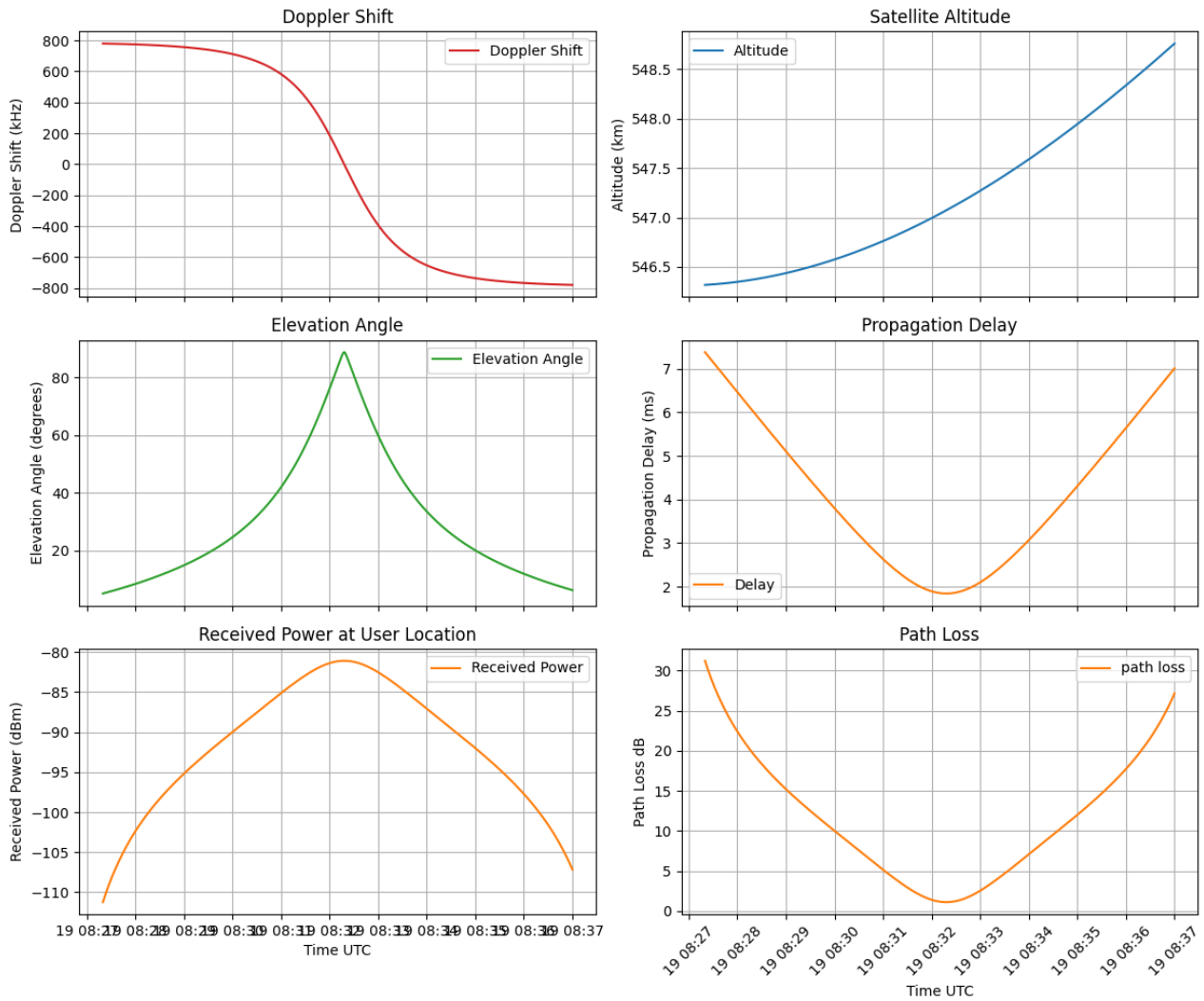
Figure 20: Example Plot at 35 GHz
