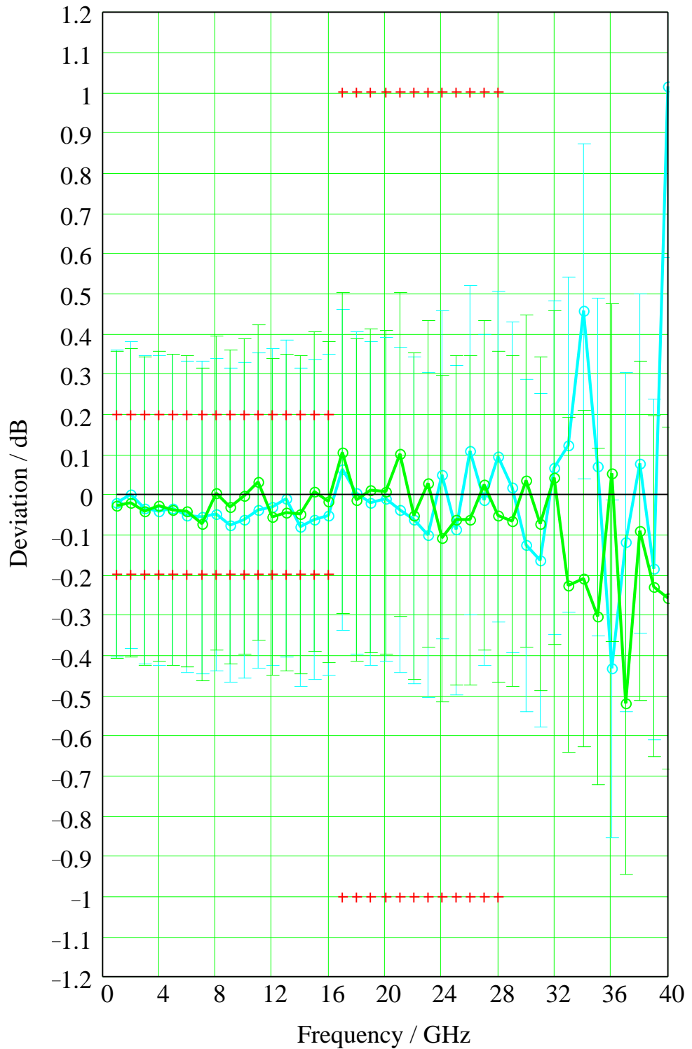
Fig. 4-11 Transmission magnitude deviations: 2.92 mm 50 dB attenuation standard
