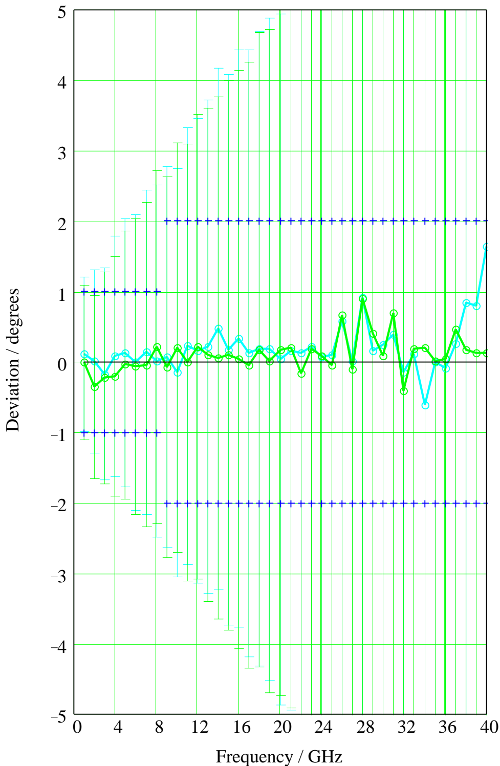
Fig. 4-20 Transmission phase deviations: 2.92 mm stepped airline verification standard
