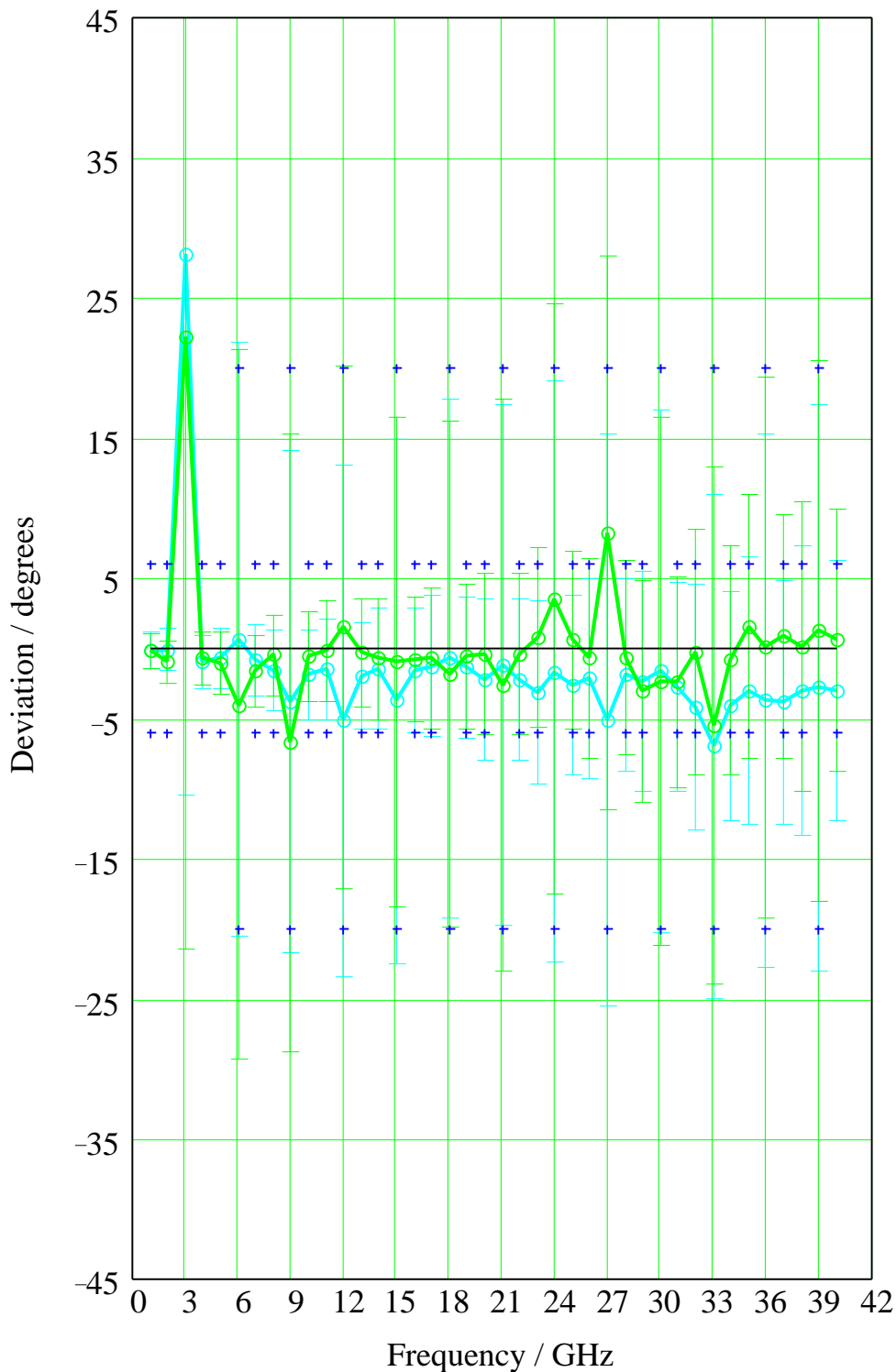
Fig. 5-5 Reflection phase deviations: stepped airline verification standard
